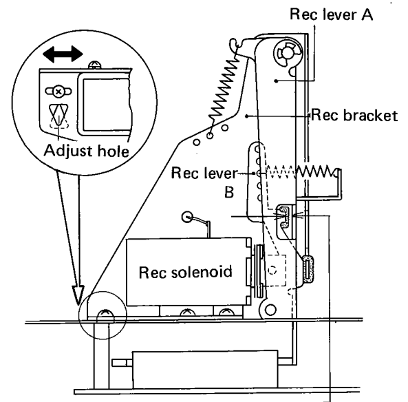
Gap (0.5–0.7 mm)
