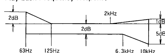
Record/Playback Frequency Response NORMAL, DOLBY(OFF)
