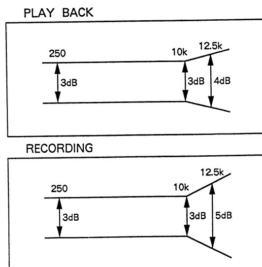
Fig. 9-5. Allowable playback frequency response zone
