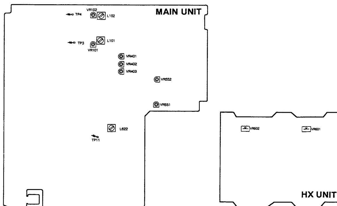
Fig. 8-2 Adjusting points
