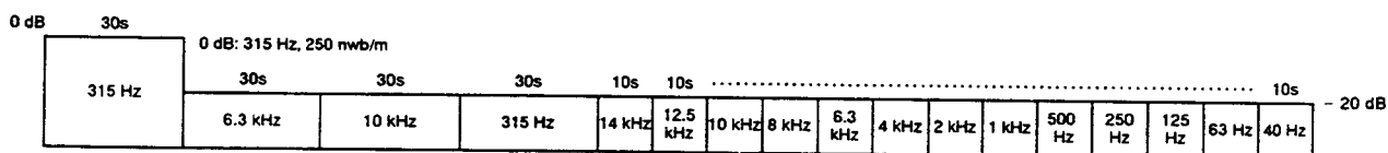
Fig. 8-3 Constants of the test tape STD-331E
