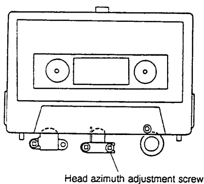
Fig. 8-4 Head azimuth adjustment
