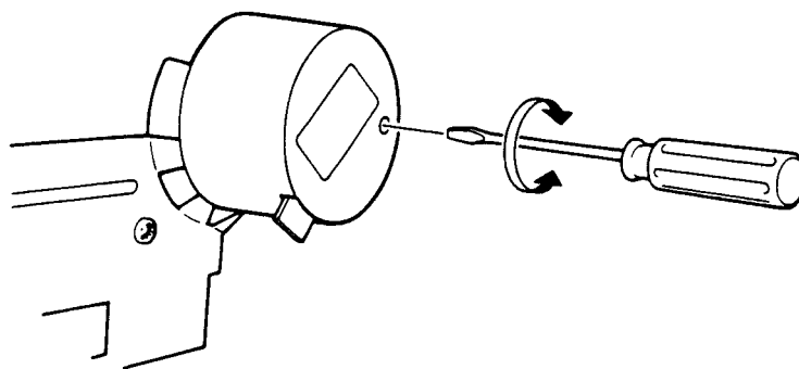
Fig. 6-1 Tape Speed Adjustment
