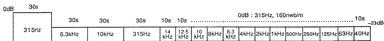
Fig. 6-3 Constants of the test tape STD-331B
