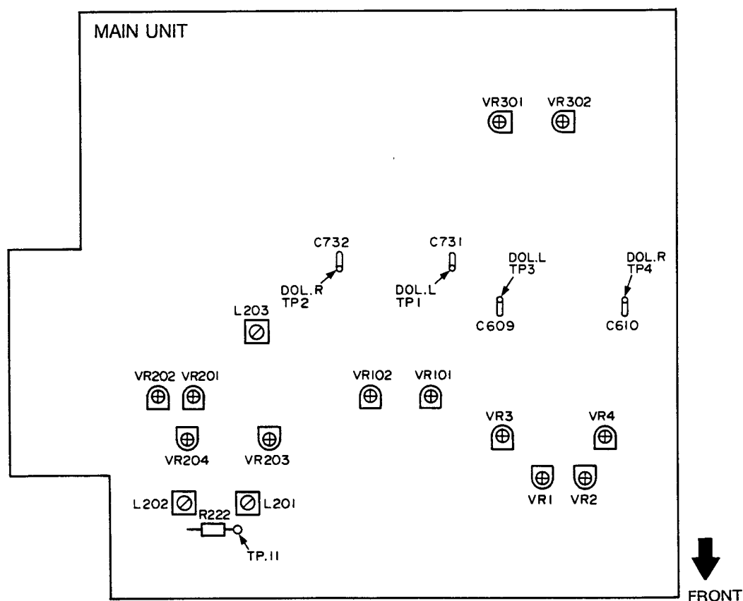
Fig. 6-2 Adjustment Locations
