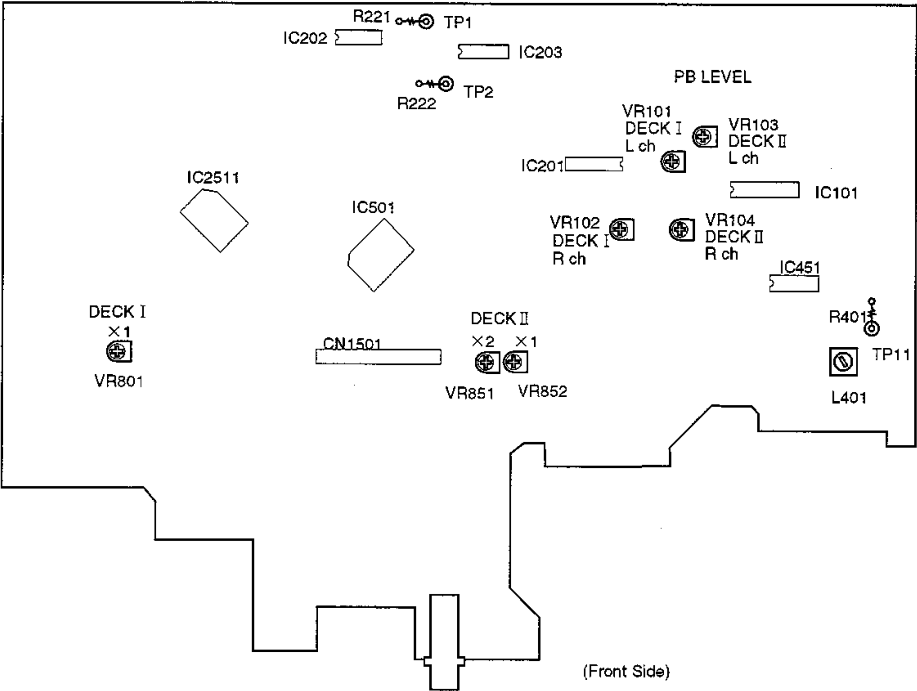
Fig. 6-6 Adjustment Points and Measurement Points
