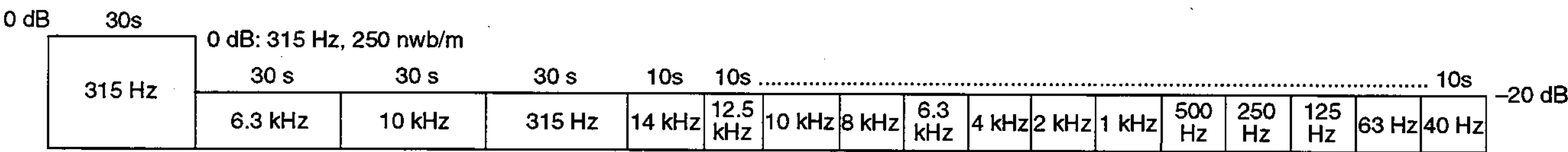
Fig. 6-2 Constants of the Test Tape STD-331E
