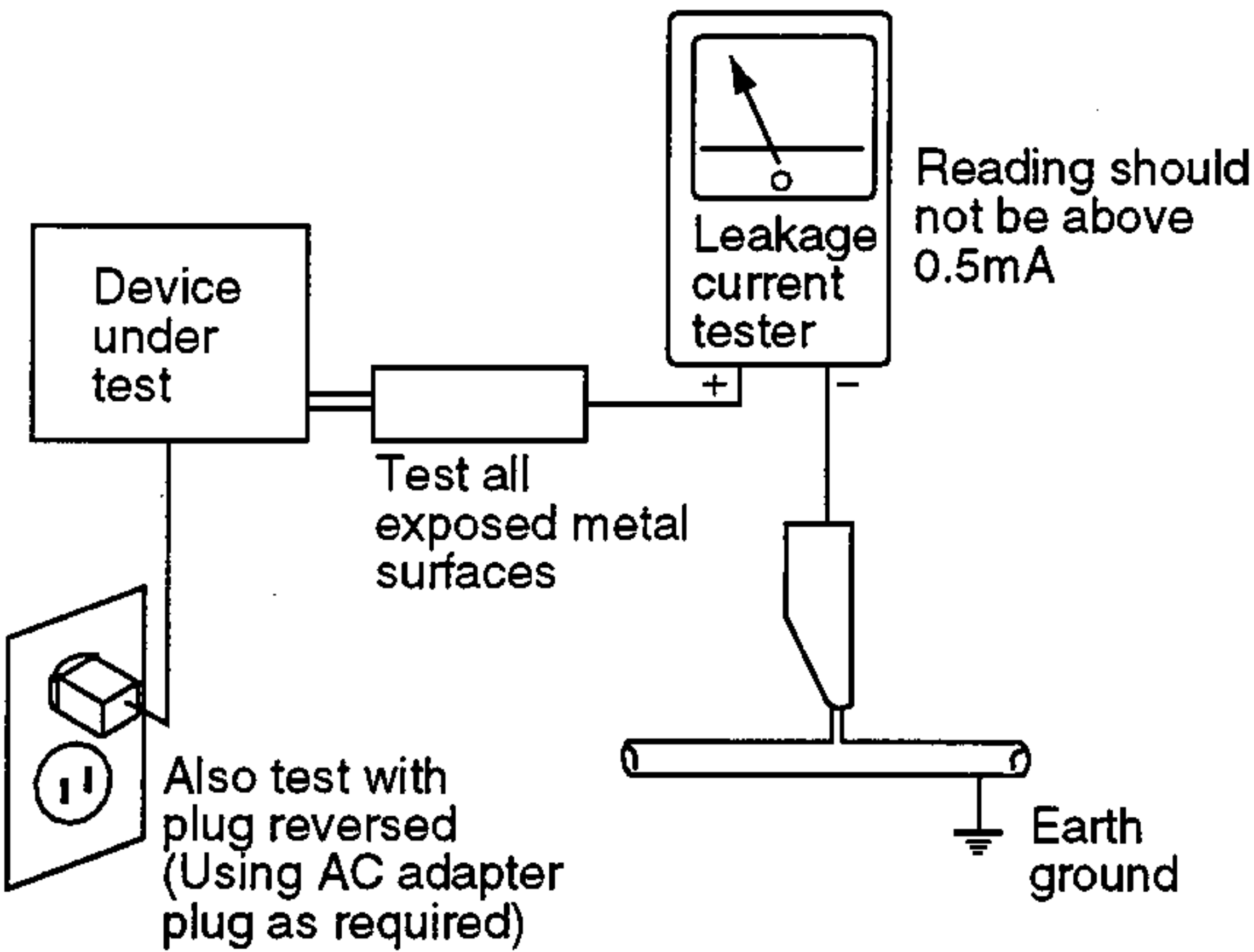
AC Leakage Test
