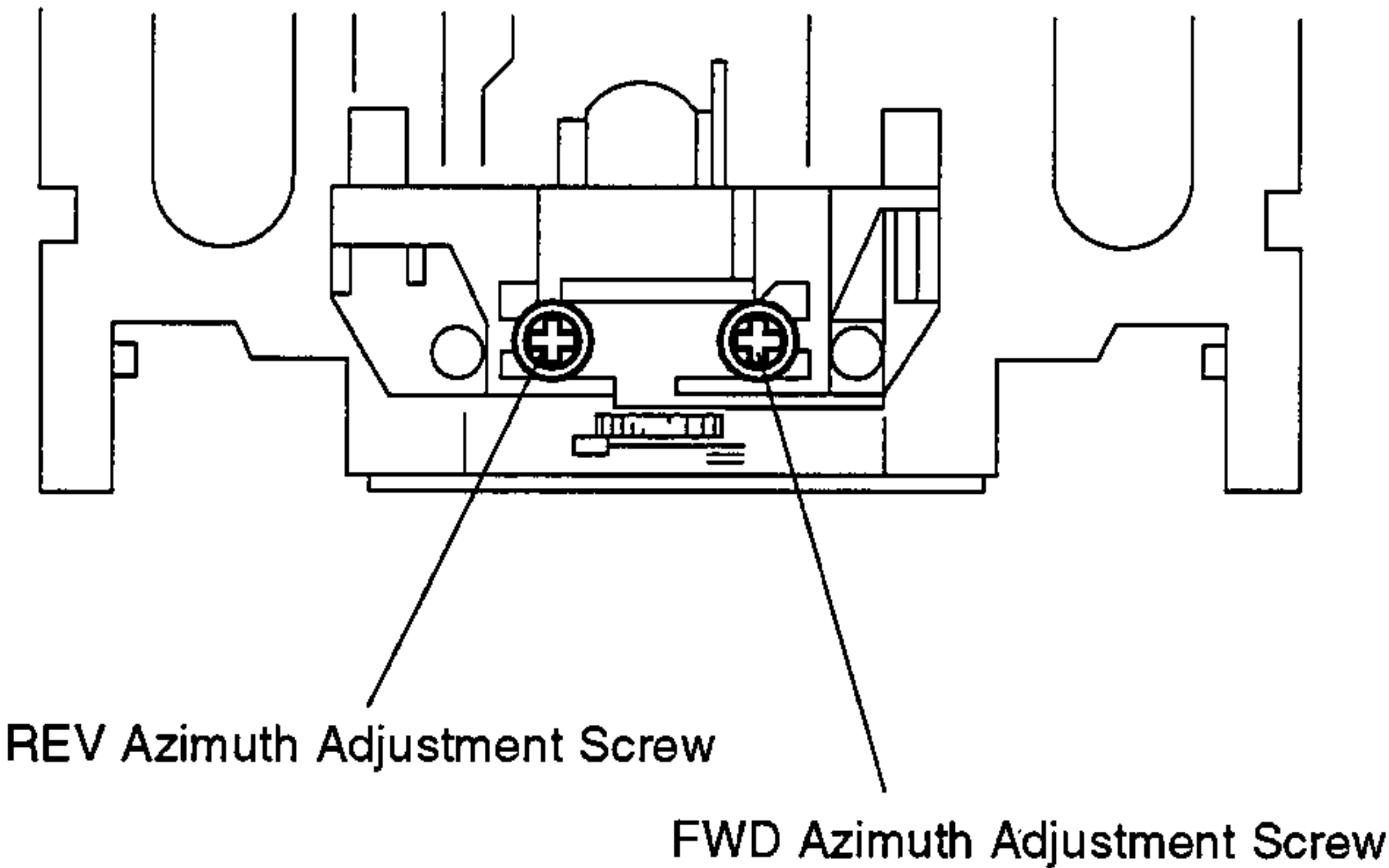
Fig. 6-3 Head Azimuth Adjustment
