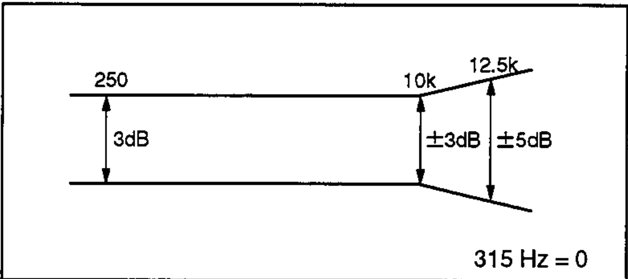
Fig. 6-4 Frequency Response Zone
