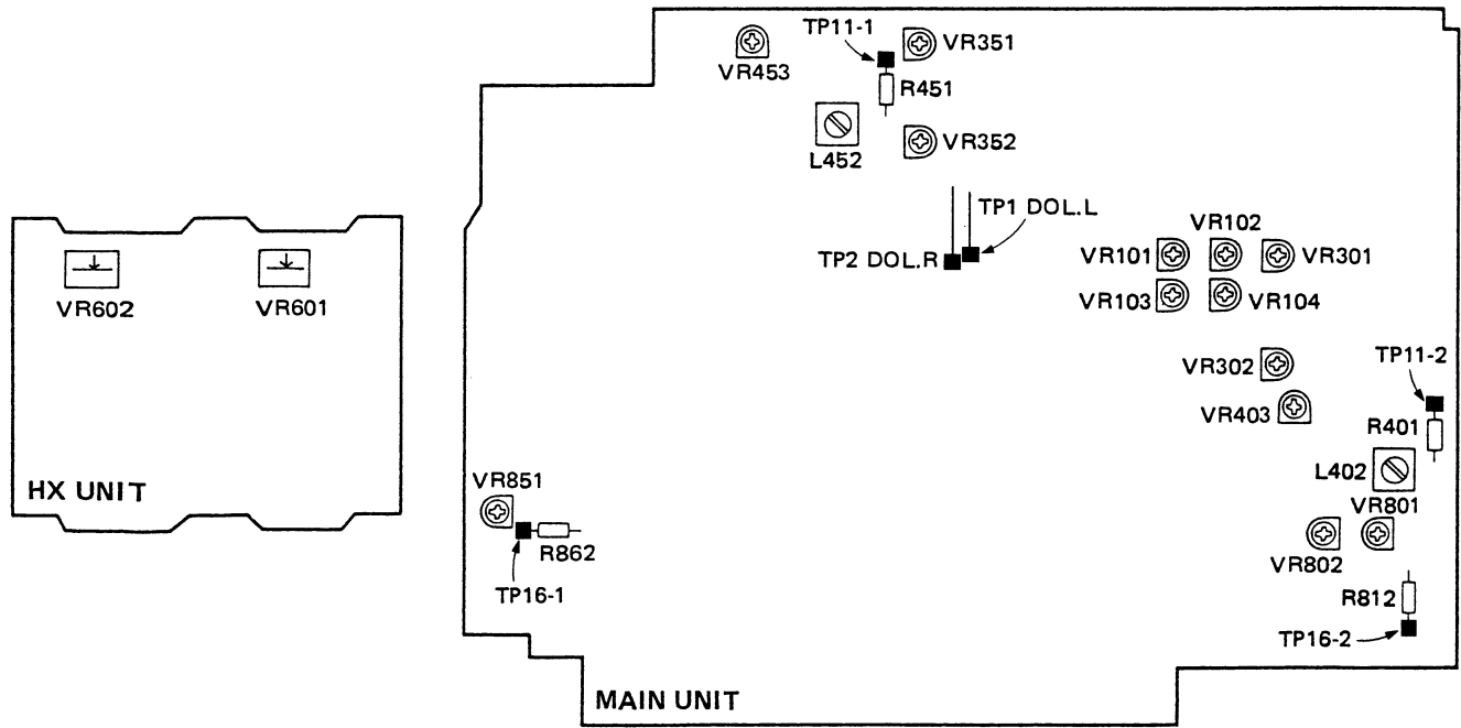
Fig. 7-1 Adjusting points
