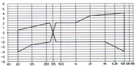
Fig. 11-9 Allowable recording and playback frequency response zone (NORM)
