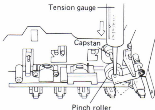
Fig. 11-1 Pinch roller pressure adjustment
