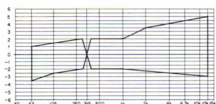
Fig. 11-11 Allowable recording and playback frequency response zone (METAL)
