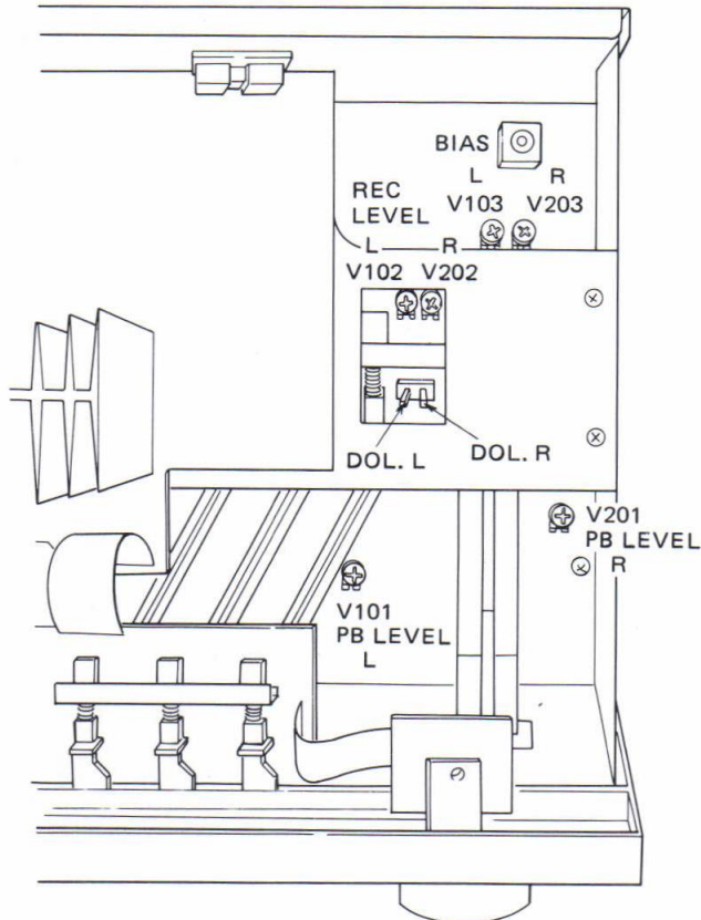
Fig. 11-8 Adjustments location
