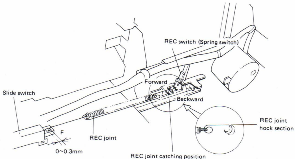
Fig. 11-4 Rec joint check and adjustment
