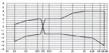
Fig. 11-10 Allowable recording and playback frequency response zone (CrO 2 )
