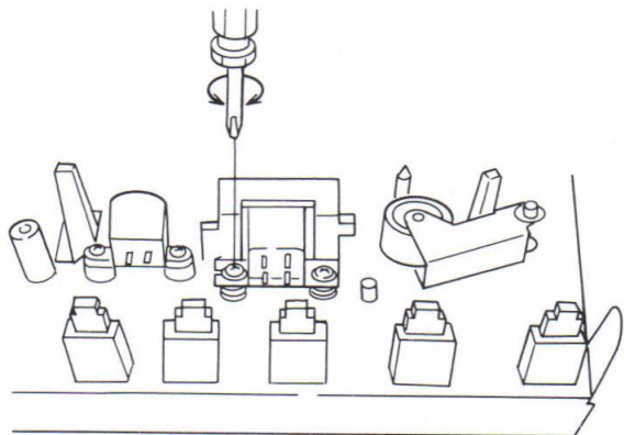
Fig. 11-6 Head azimuth adjustment
