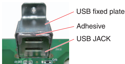
USB fixed plate for the initial products
