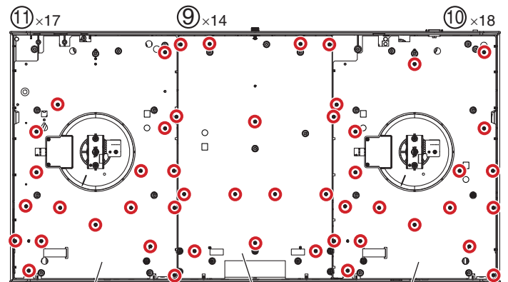
CONTROL PCB Assy B
