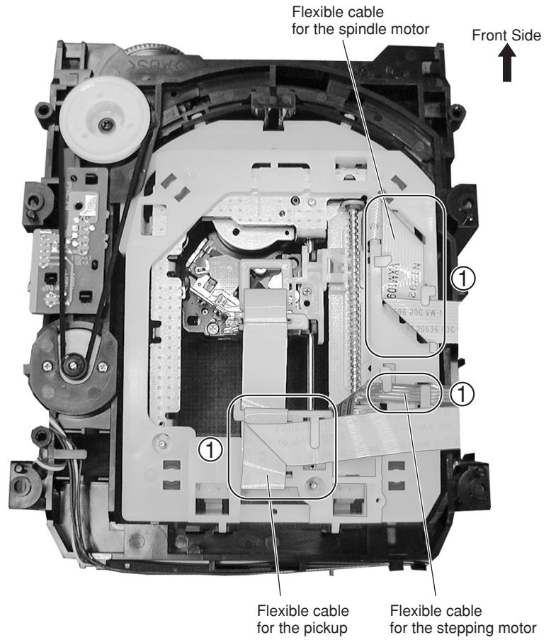
● Bottom View
