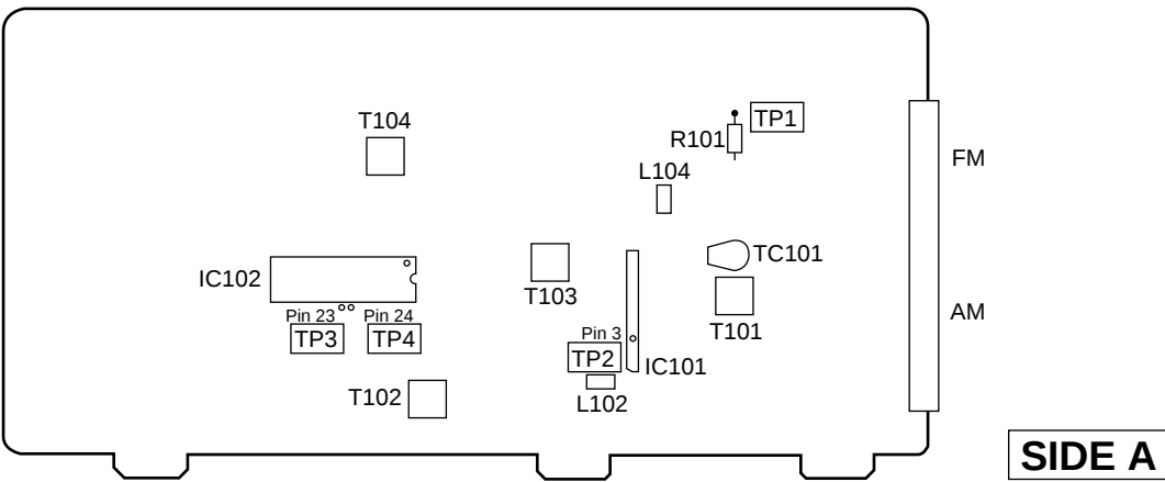
Fig.6 Adjustment Point
