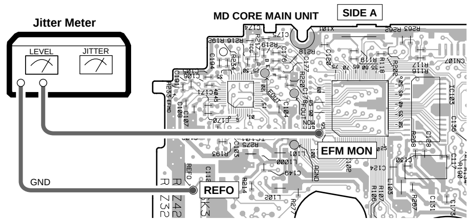
Connection diagram
