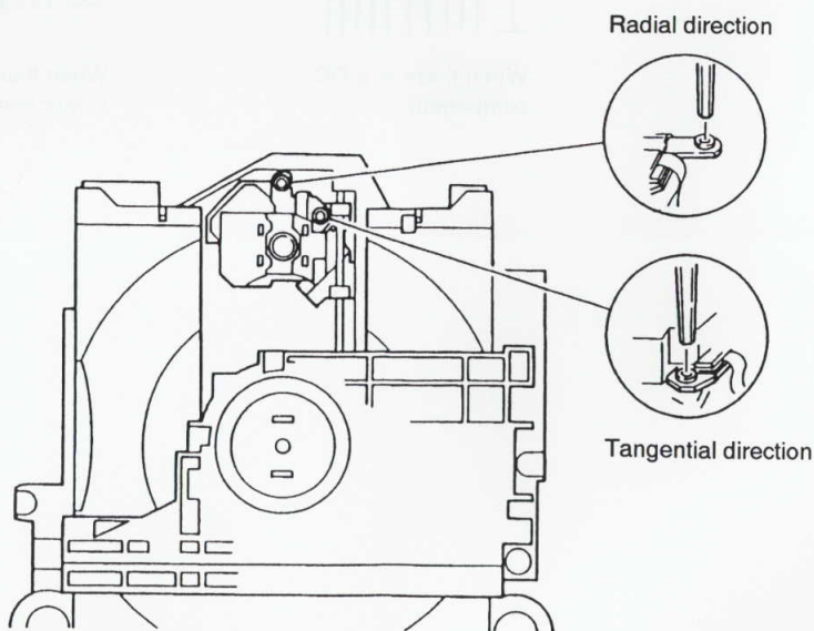
Adjustment Locations
