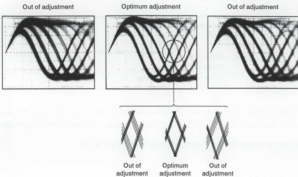
Figure 5 Eye pattern
