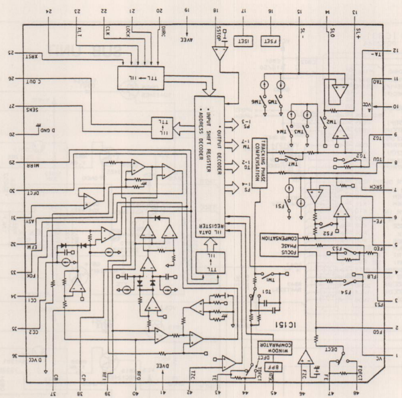
CXA1372Q
