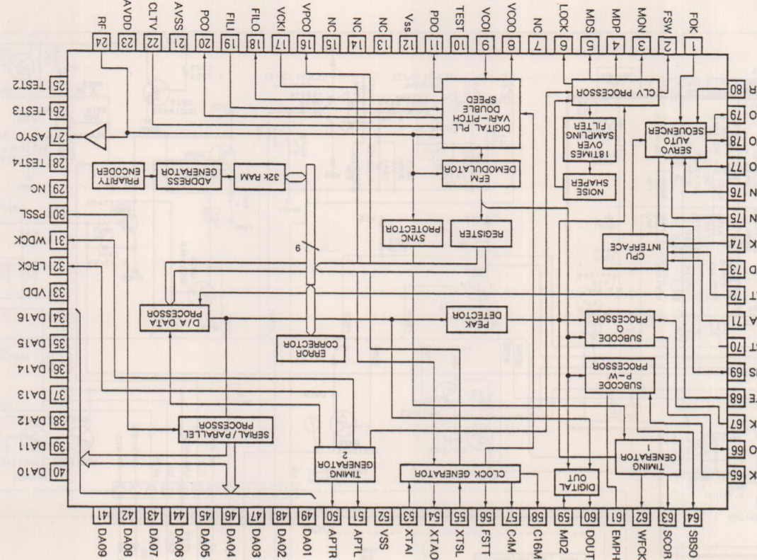
CXD2500AQ
