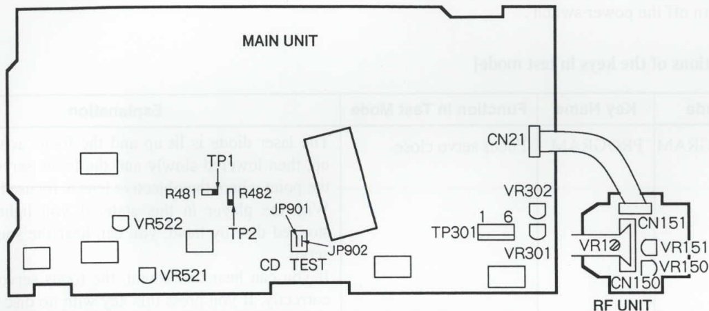
Figure 1 Adjustment Locations
