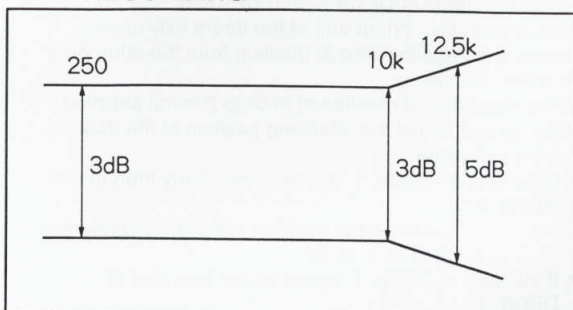
Fig. 6 Frequency response
