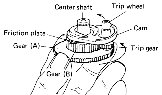
Fig. 11-2 Gear cluster
