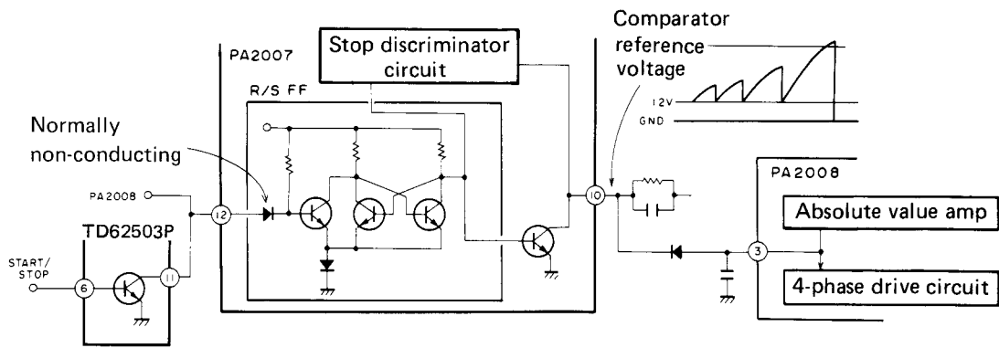
Fig. 12-6 Stop discriminator theoretical circuit
