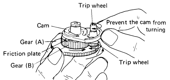
Fig. 11-3 Gear cluster operation
