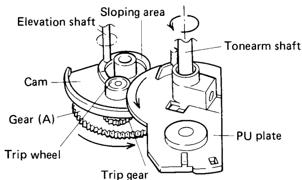
Fig. 11-5 Return operation
