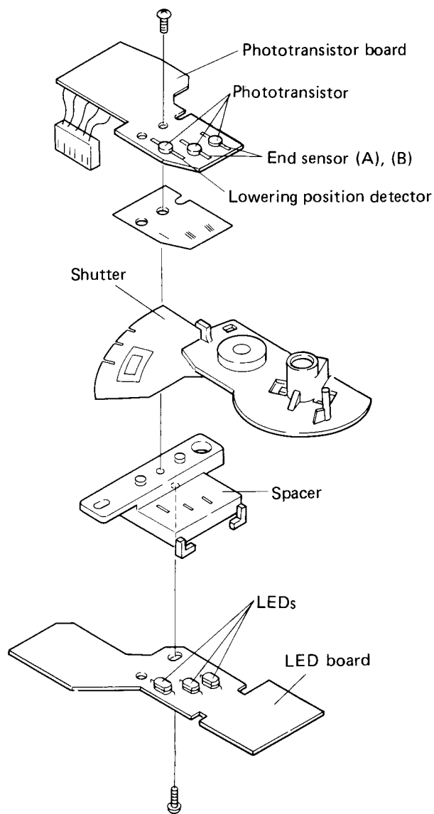
Fig. 11-6 Sensing mechanism
