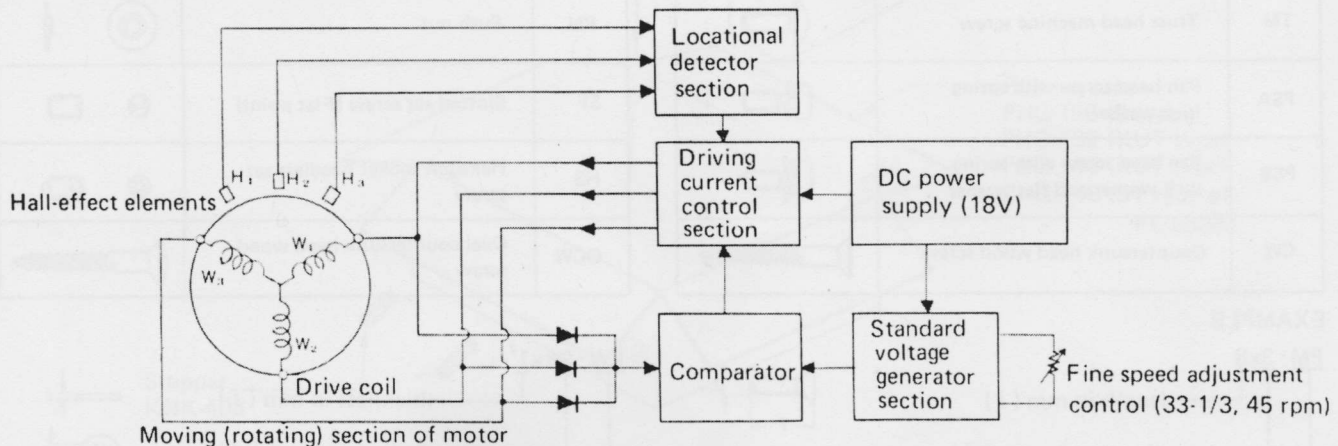
Fig. 2: Block Diagram of the PXM-020
