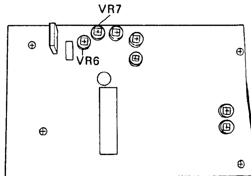
Fig. 6-8 Lead-in and return speed adjustment
