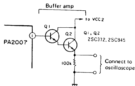
Fig. 6-9 Connect buffer amp
