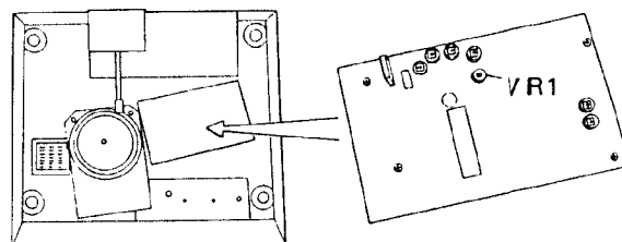
Fig. 6-3 End sensor sensitivity adjustment
