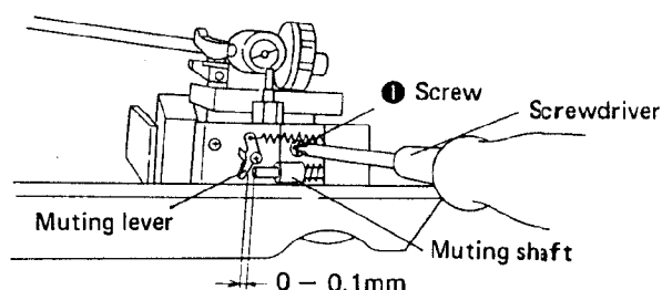
Fig. 6-2 Muting timing adjustment 2
