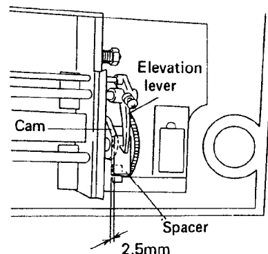
Fig. 6-1 Muting timing adjustment 1
