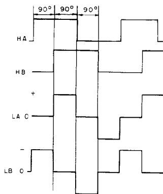
Fig. 4-12 Drive circuit waveforms
