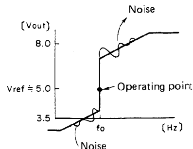
Fig. 4-7 Input/output characteristics
