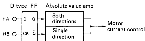
Fig. 4-13 Reverse rotation sensor equivalent circuit
