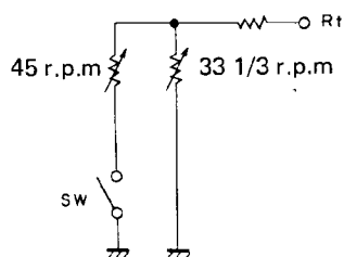
Fig. 4-5 Switching reference frequency
