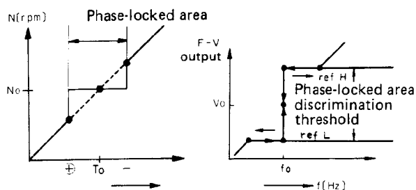
Fig. 4-8 F/V converter output
