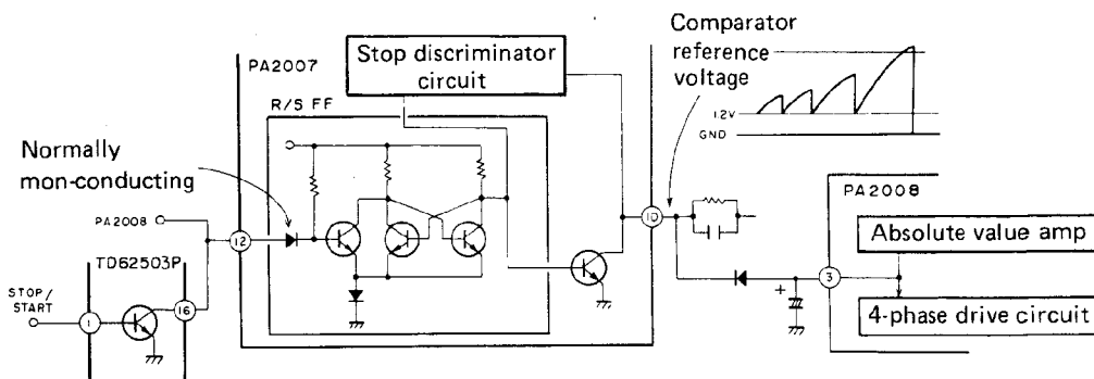
Fig. 4-10 Stop discriminator theoretical circuit
