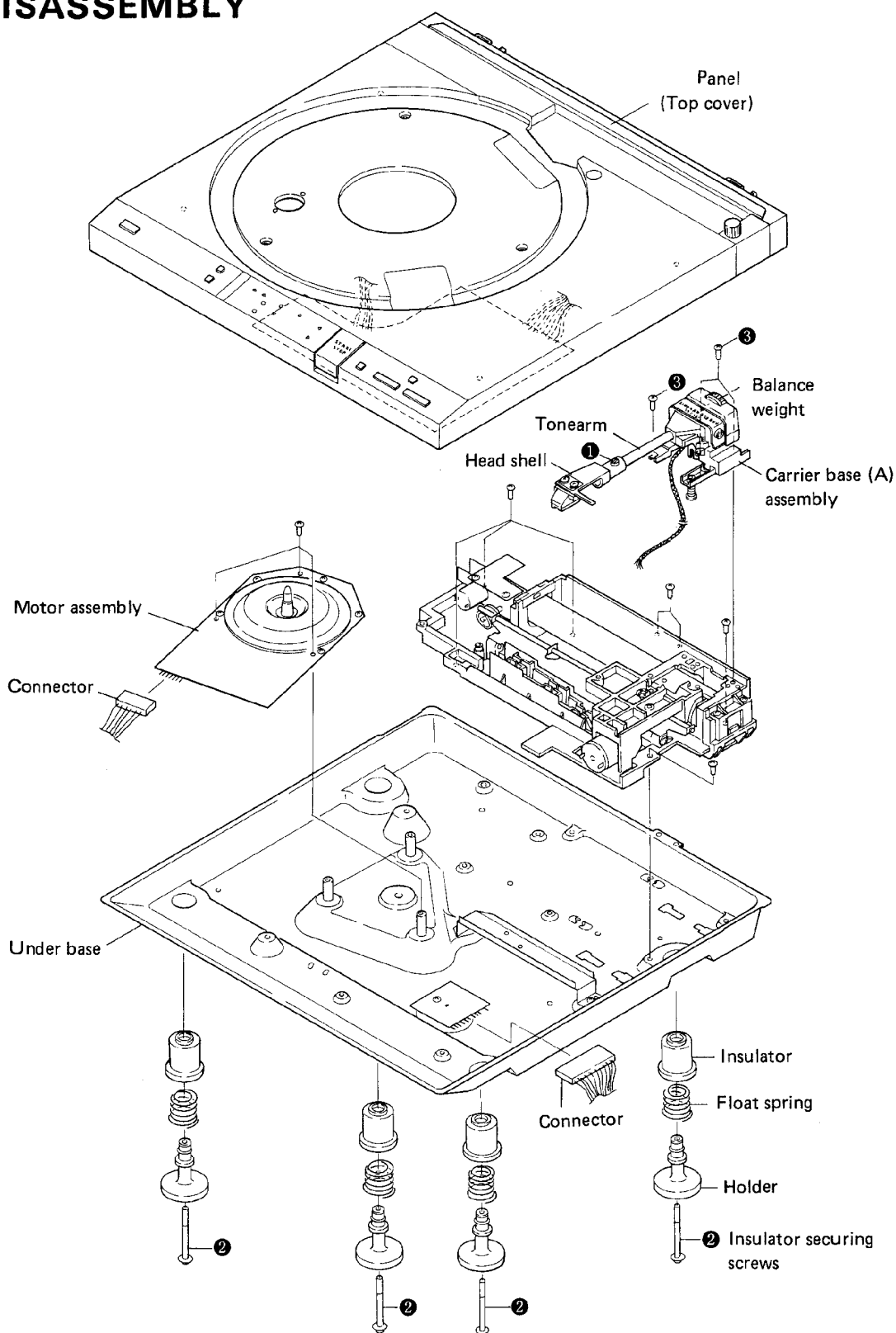
Fig. 3-1 Disassembly
