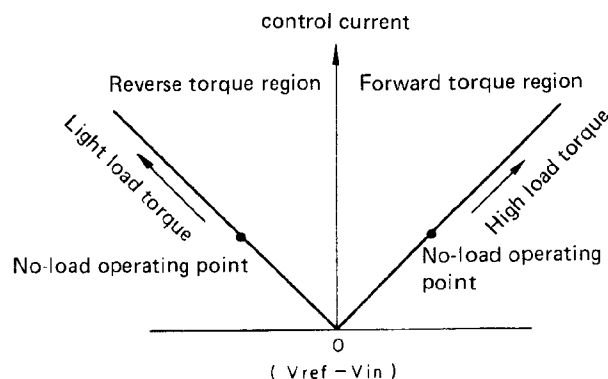
Fig. 4-11 Input/output characteristics
