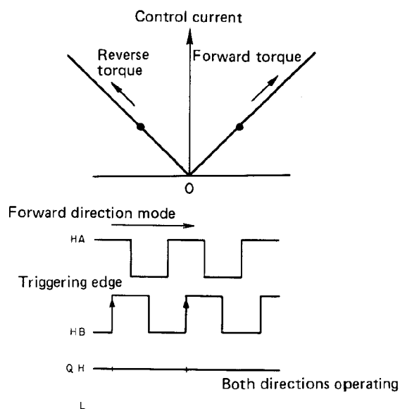
Fig. 4-14 Forward direction mode
