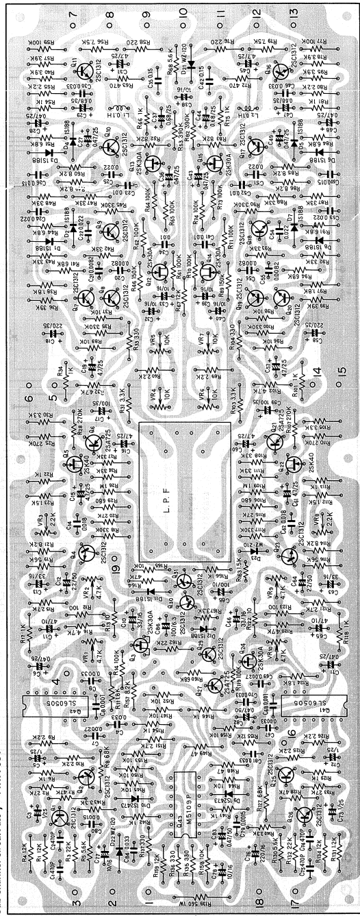
Sub channel circuit ass'y AWM-051
