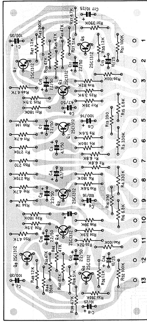
Matrix ass'y AWM-048
