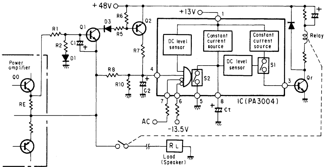
Fig. 6-5 Protection circuit
