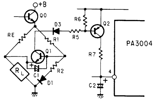
Fig. 6-6 Overload detector
