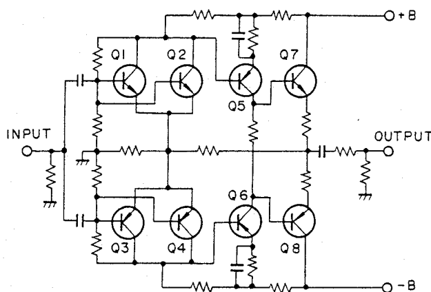
Fig. 5-2 MC Amplifier
