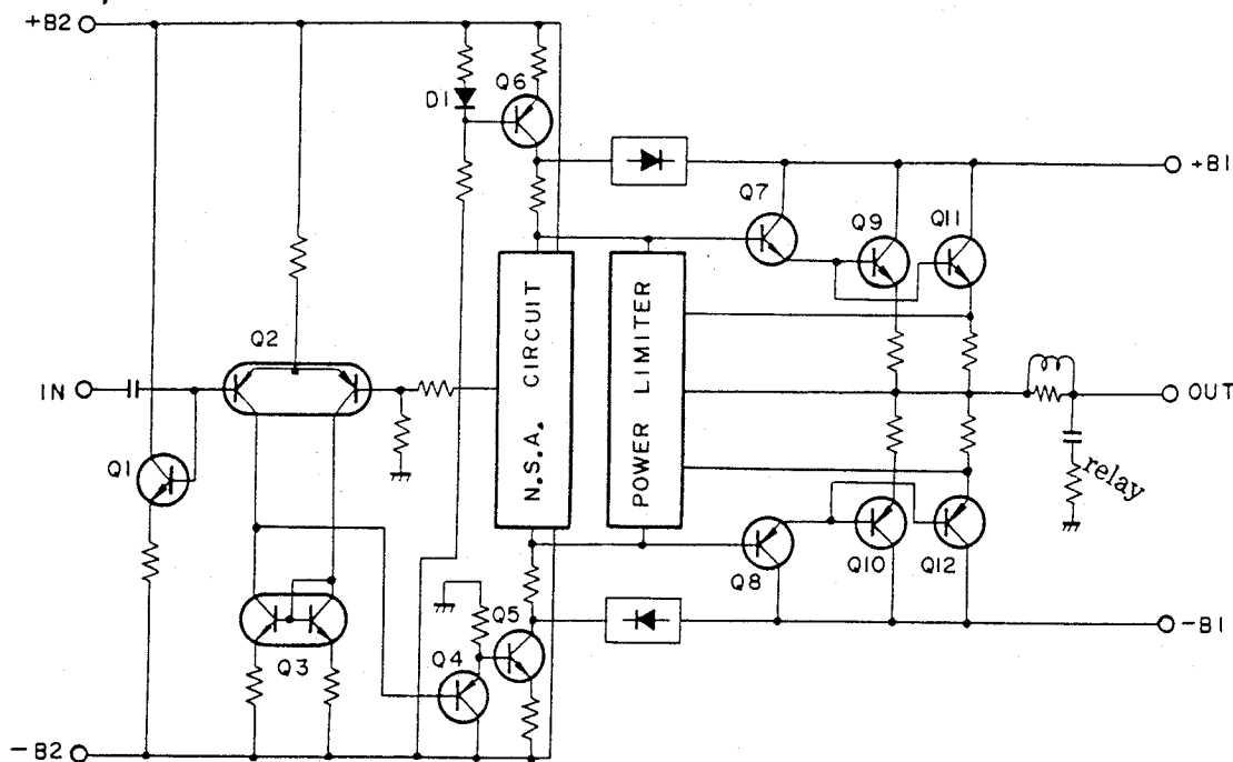
Fig. 5-5 Power Amplifier
