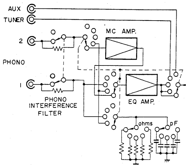
Fig. 5-1 Phono Circuit
