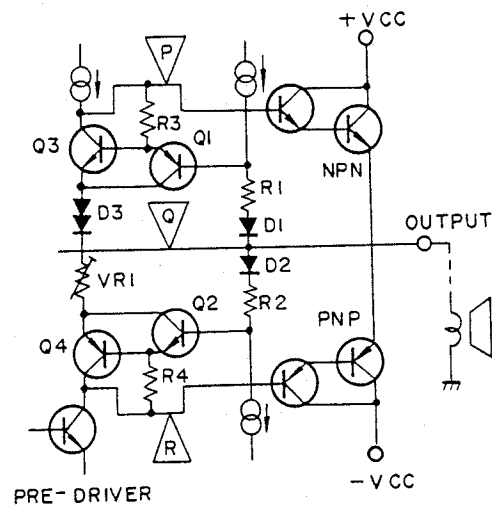
Fig. 5-9 NSA Circuit
