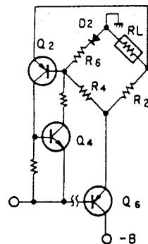
Fig. 5-7 Bridge Circuit
