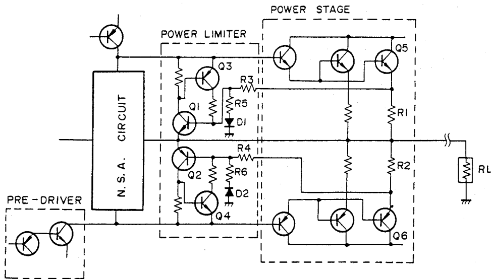
Fig. 5-6 Power Limiter
