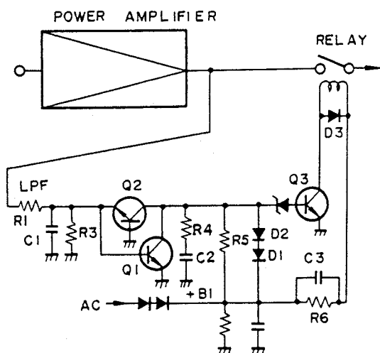
Fig. 5-13 Protection Circuit
