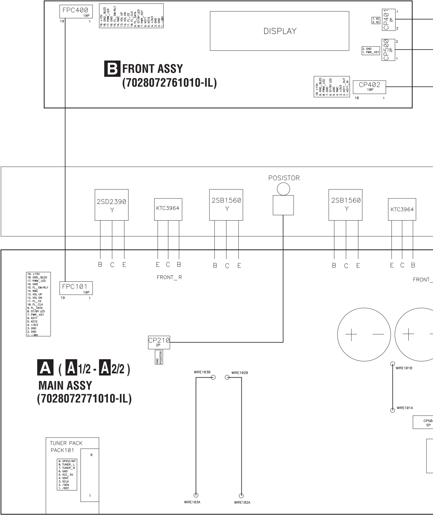
SX-20 WIRING DIAGRAM
