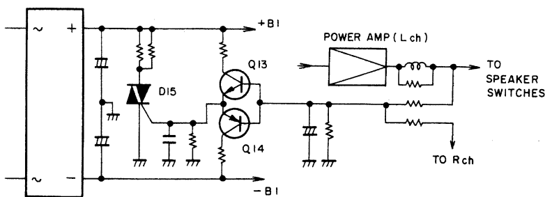
Fig. 5-2 DC Voltage protection circuit
