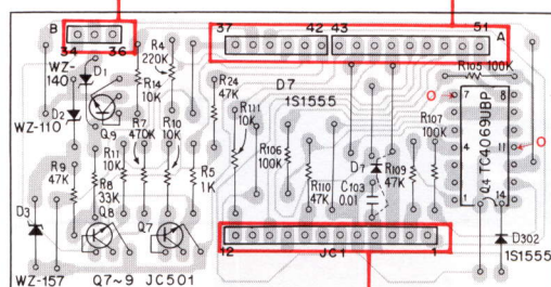
CONTROL Ass'y B (GWX-717)
