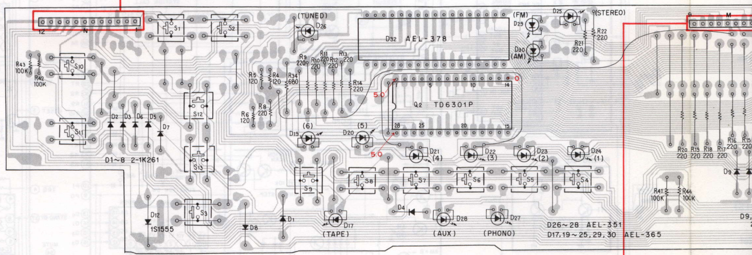
CONTROL Ass'y(GWX-706)
