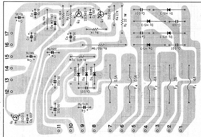
Power supply ass'y AWR-065
