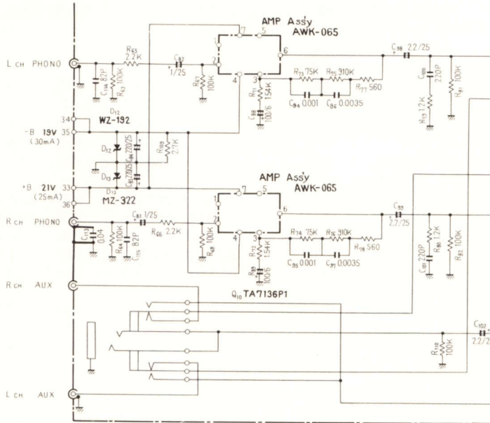
AWK-065 PCB
