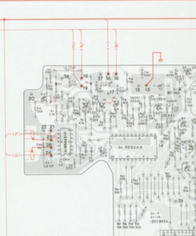
READ OUT Ass'y (AWV-011)
