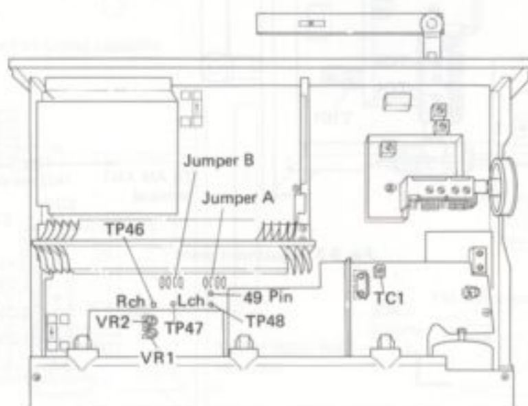
Fig. 8-4 Adjustment point
