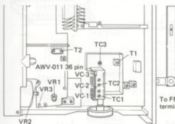
Fig. 8-2 Adjustment point
