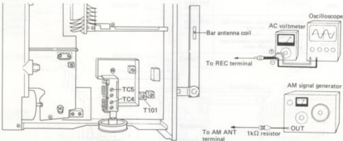
Fig. 8-3 Adjustment point
