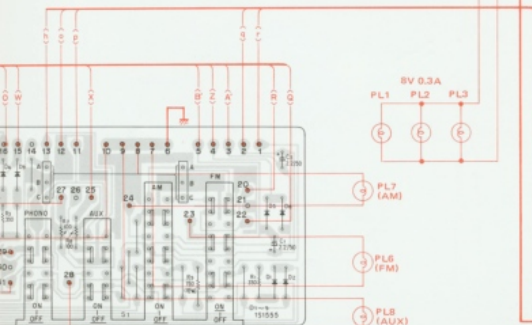
Ass'y (AWS-149)
