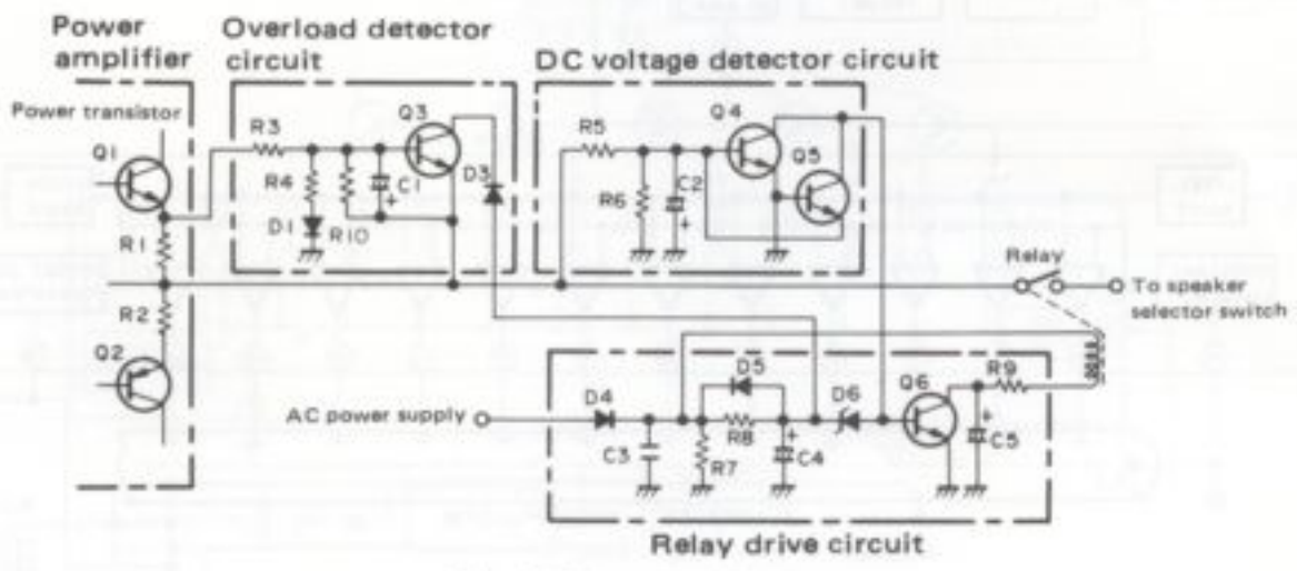
Fig. 4-11 Protection Circuit
