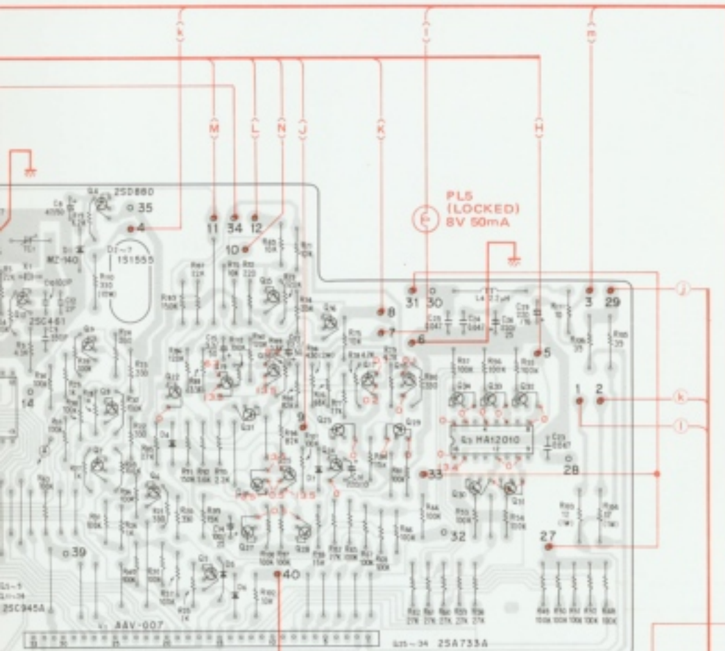
Ass'y (AWV-011)
