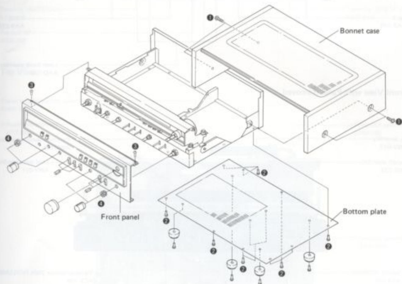
Fig. 5-1 Disassembly
