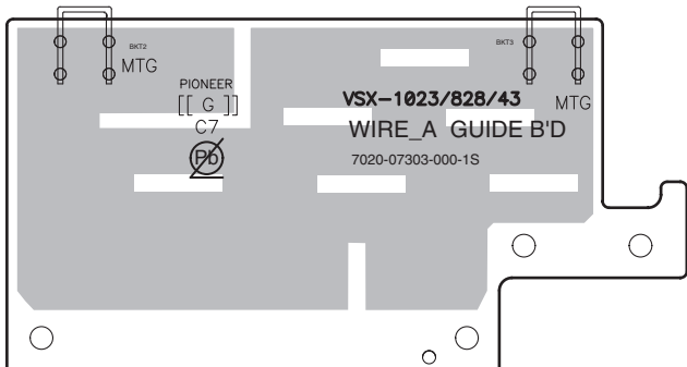
WIRE-A ASSY
