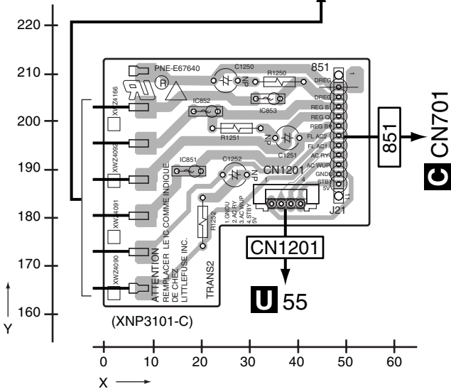
TRANS2 ASSY
