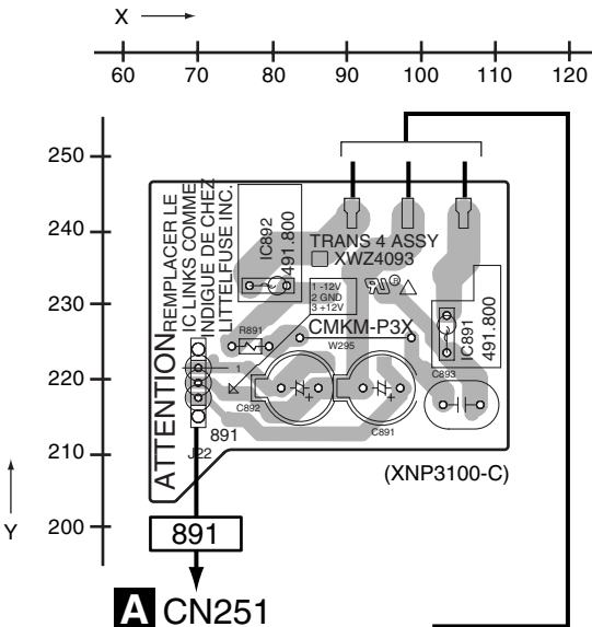
TRANS4 ASSY
