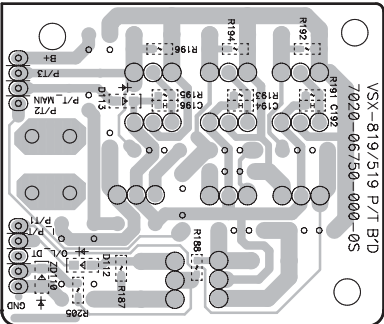
B P.C.B SUB ASSY (P/T)
