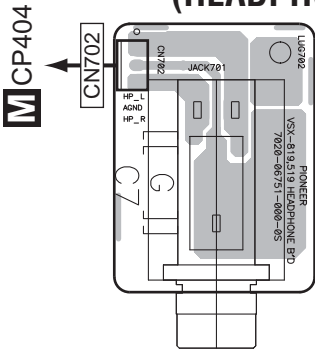
F P.C.B SUB ASSY (HEADPHONE)
