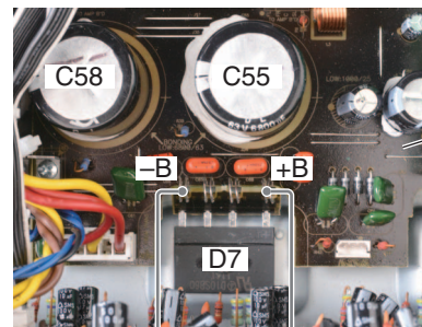
MAIN Assy
