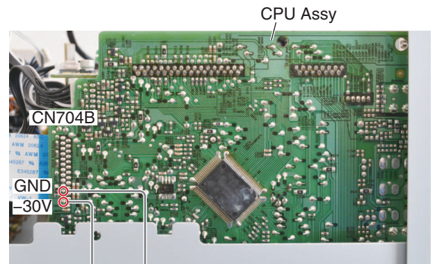
CPU Assy
