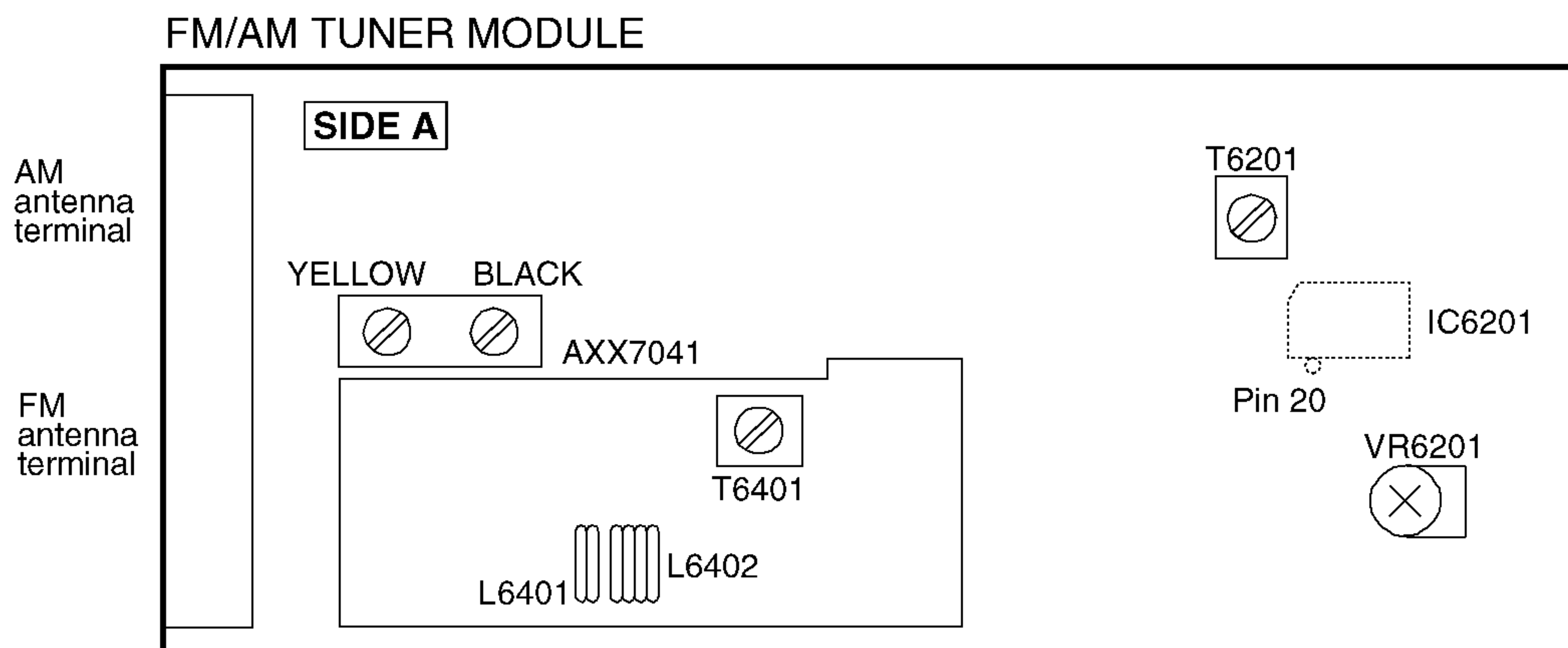
Fig. 2 Adjustment Point
