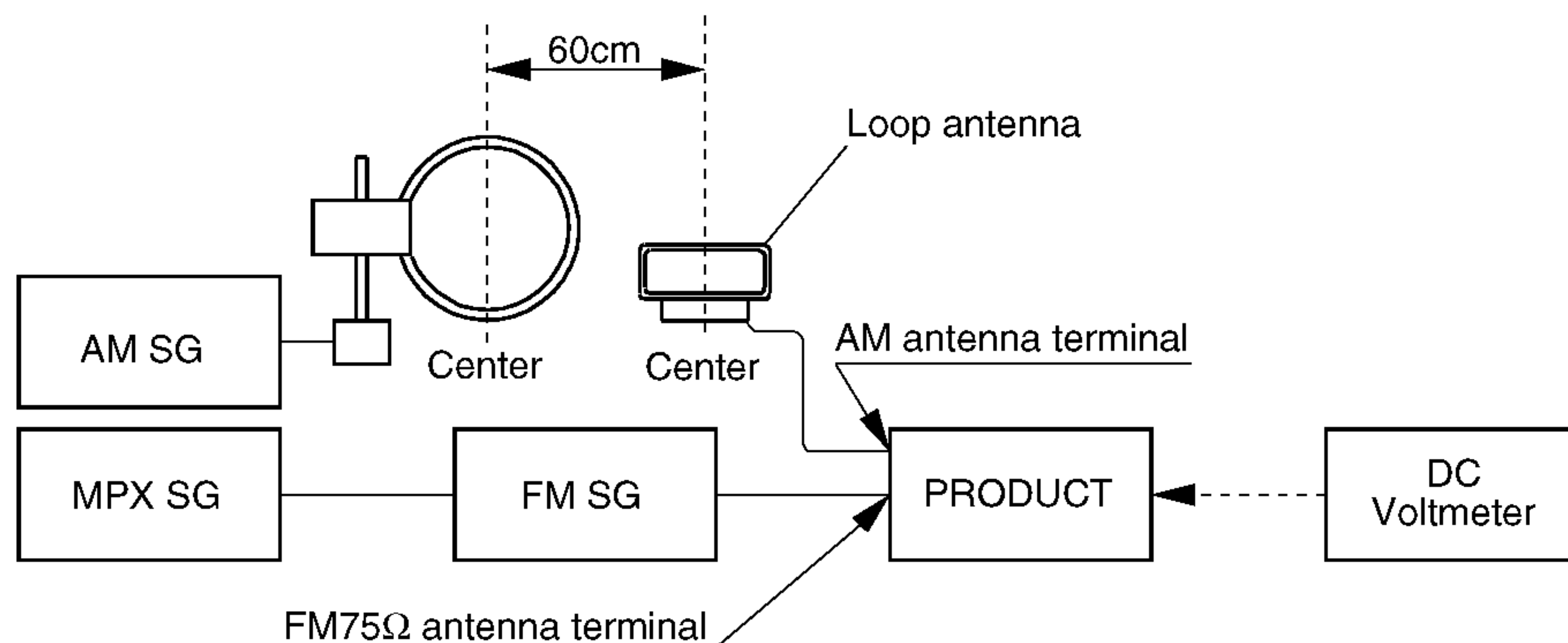
Fig. 1 AM and FM Adjustment Wiring Diagram
