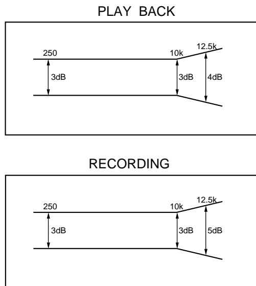
Fig. 6 Frequency Characteristics
