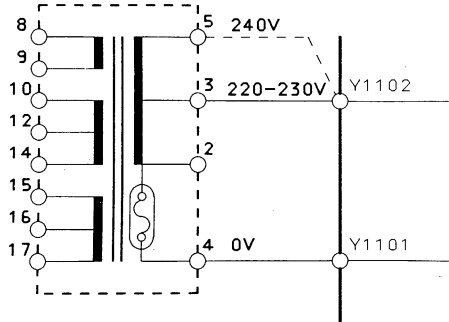
T8005 ATS7011 POWER TRANSFORMER (XR-P340)
