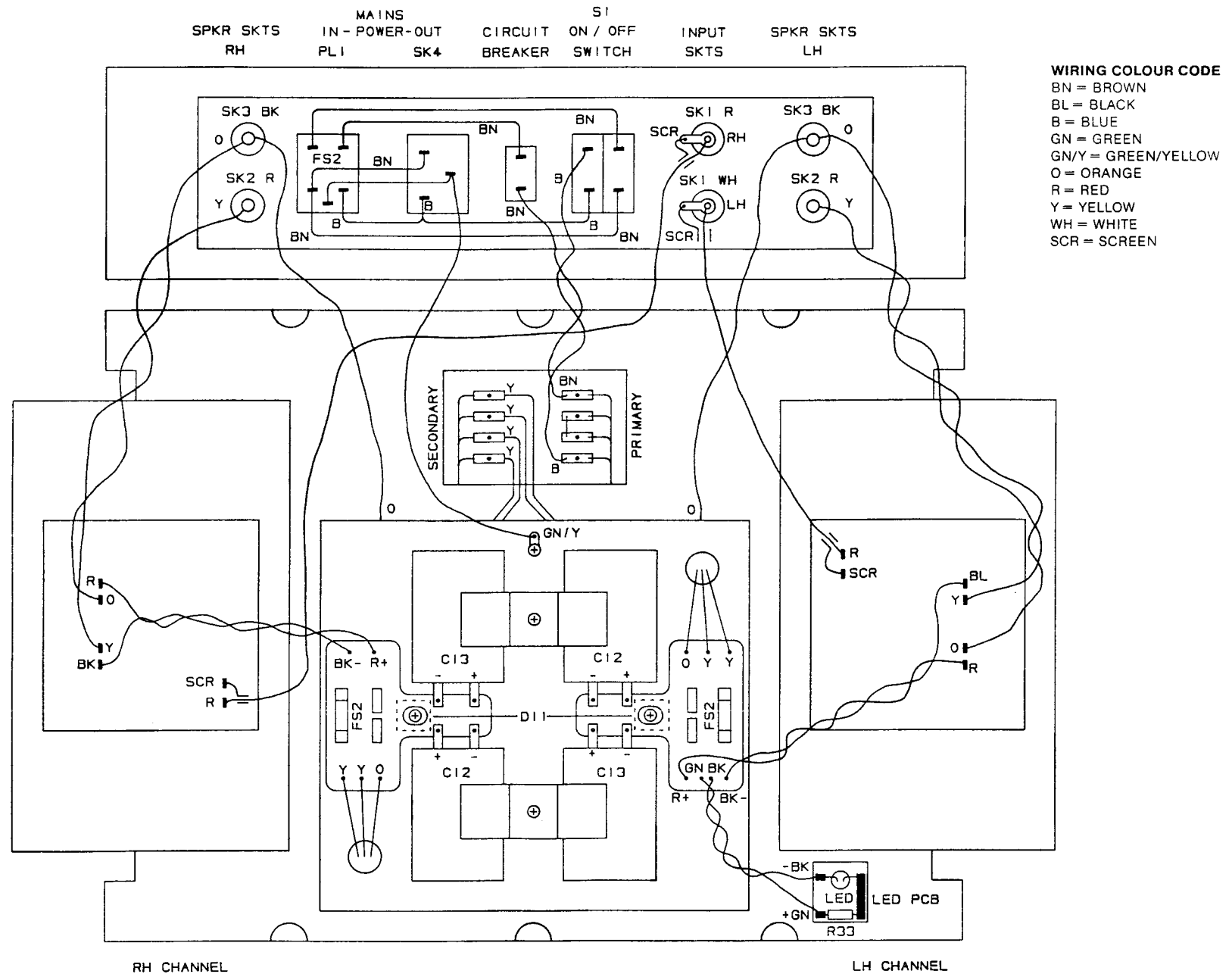
Main Wiring Layout (Bottom View)
