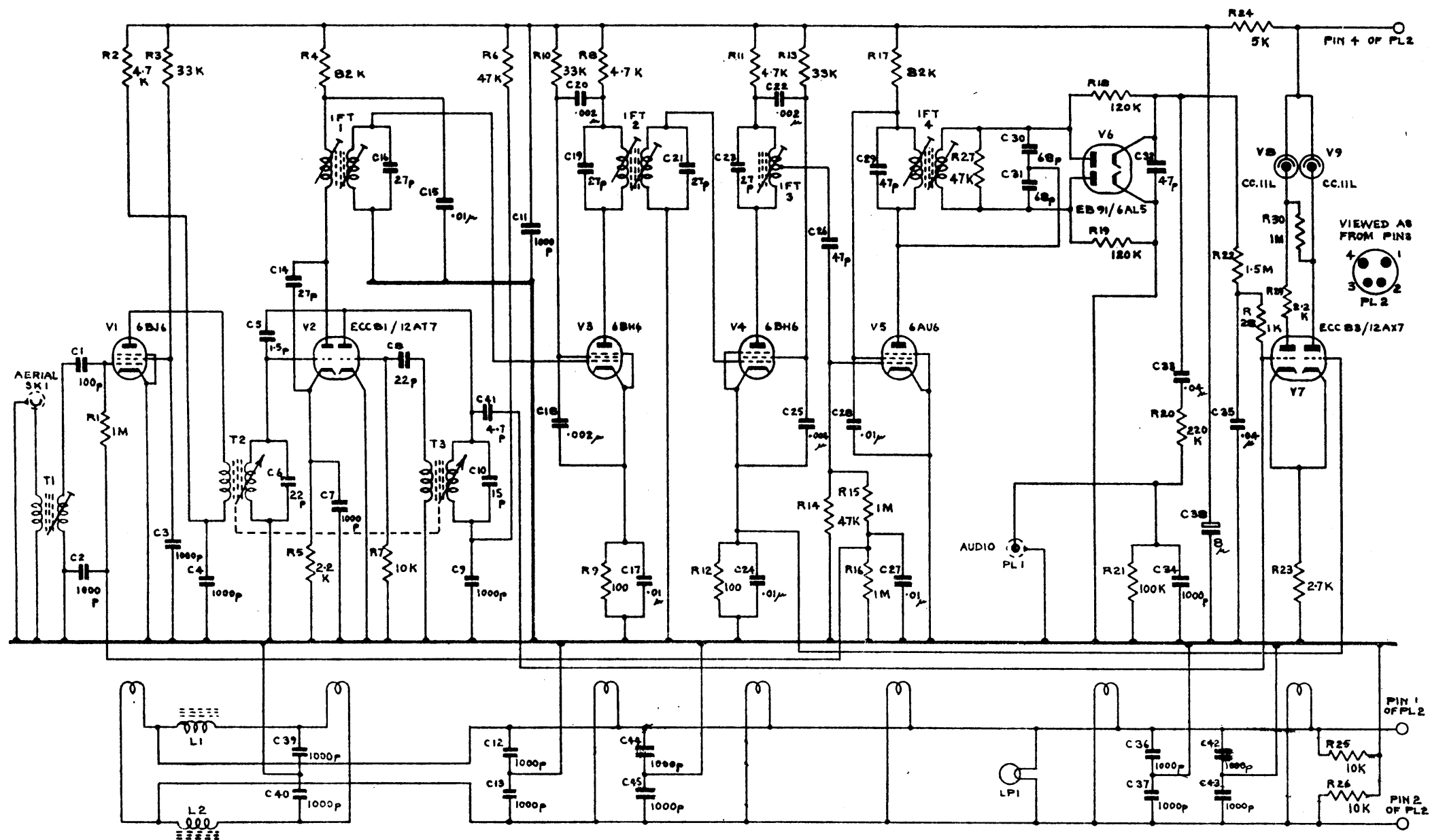
CIRCUIT DIAGRAM, F.M. TUNER, SERIES B.
