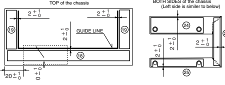
POSITIONING OF CUSHIONS ON CHASSIS(measuring scale)
