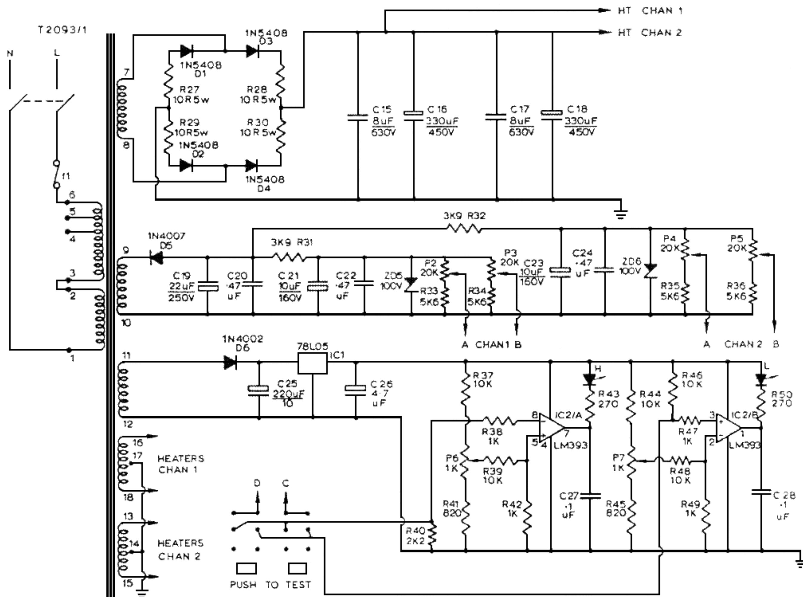
Fig.3 Power Supply Circuit STA25 Renaissance
