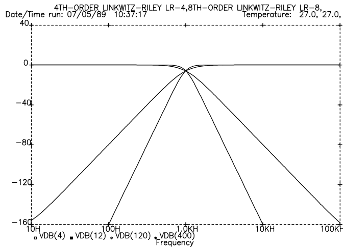
Figure 12. LR-4 and LR-8 slopes
