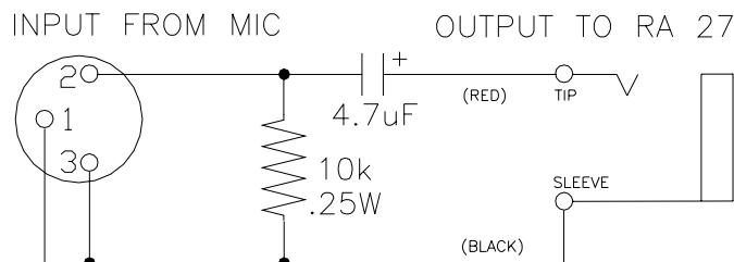
Figure 2. RA 27 Dynamic Mic Adaptor
