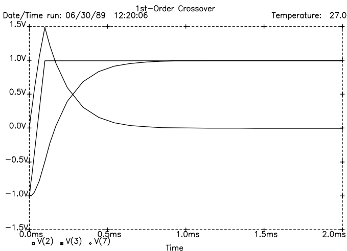
Figure 5. 1st-order transient response
