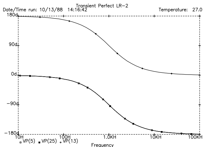
Figure 9. LR-2 phase response
