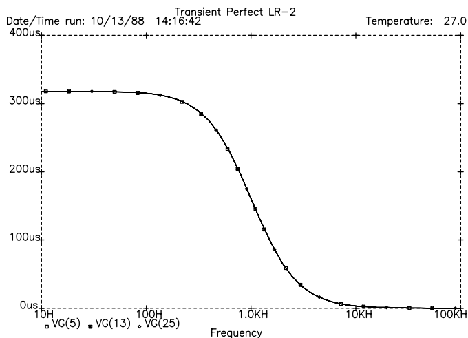
Figure 10. LR-2 group delay
