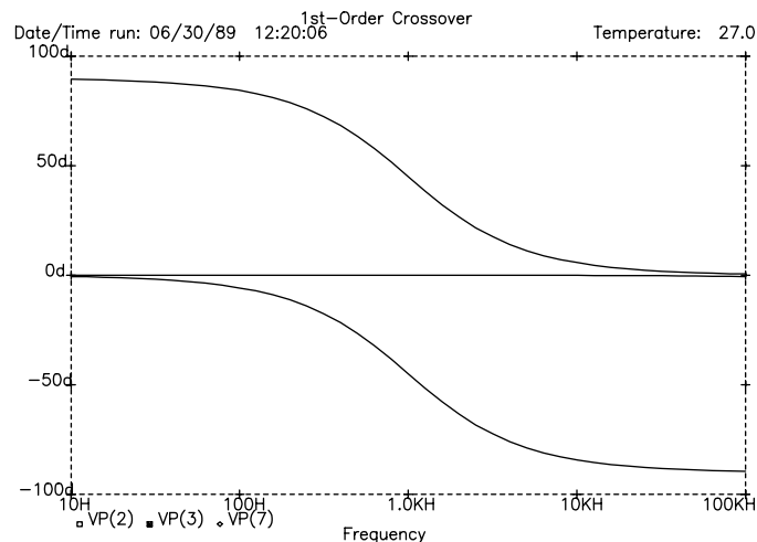
Figure 3. 1st-order response
