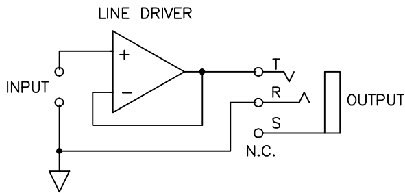
Figure 3. FLOATING UNBALANCED 1/4" TRS OUTPUT
