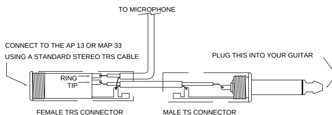
Demo Mic Adaptor Wye Cable
