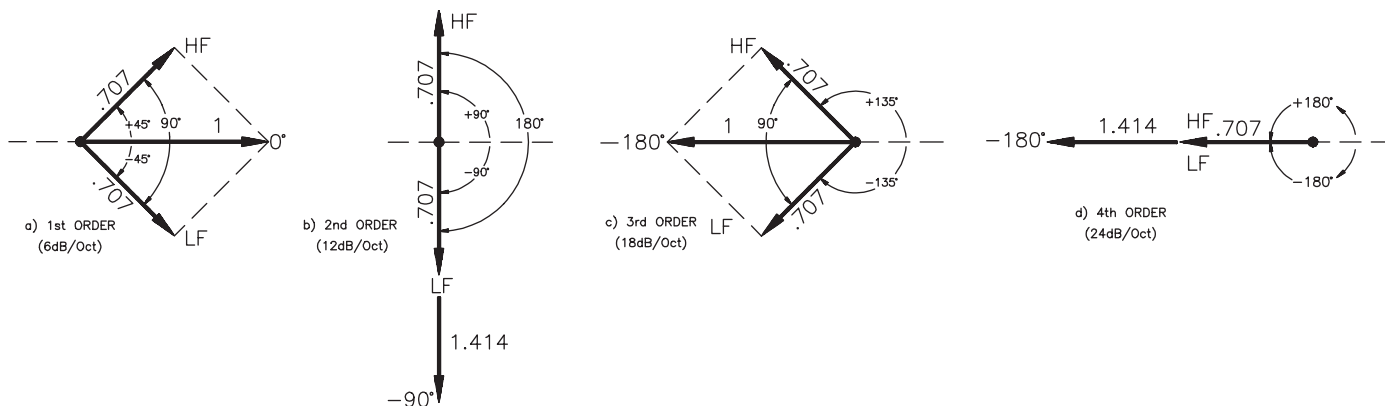
Figure 6. 1st-order Vector and 2nd through 4th-order Butterworth Vector Diagrams
