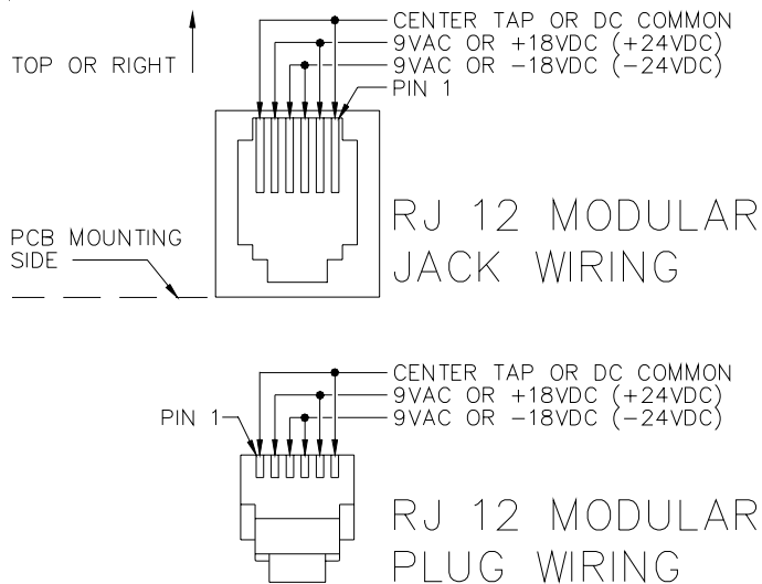
Figure 1. RJ 12 Modular Jack & Plug Wiring
