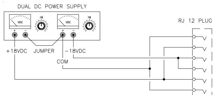
Figure 4. DC Power Supply Wiring
