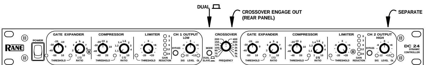
"Straight Wire" Setup
