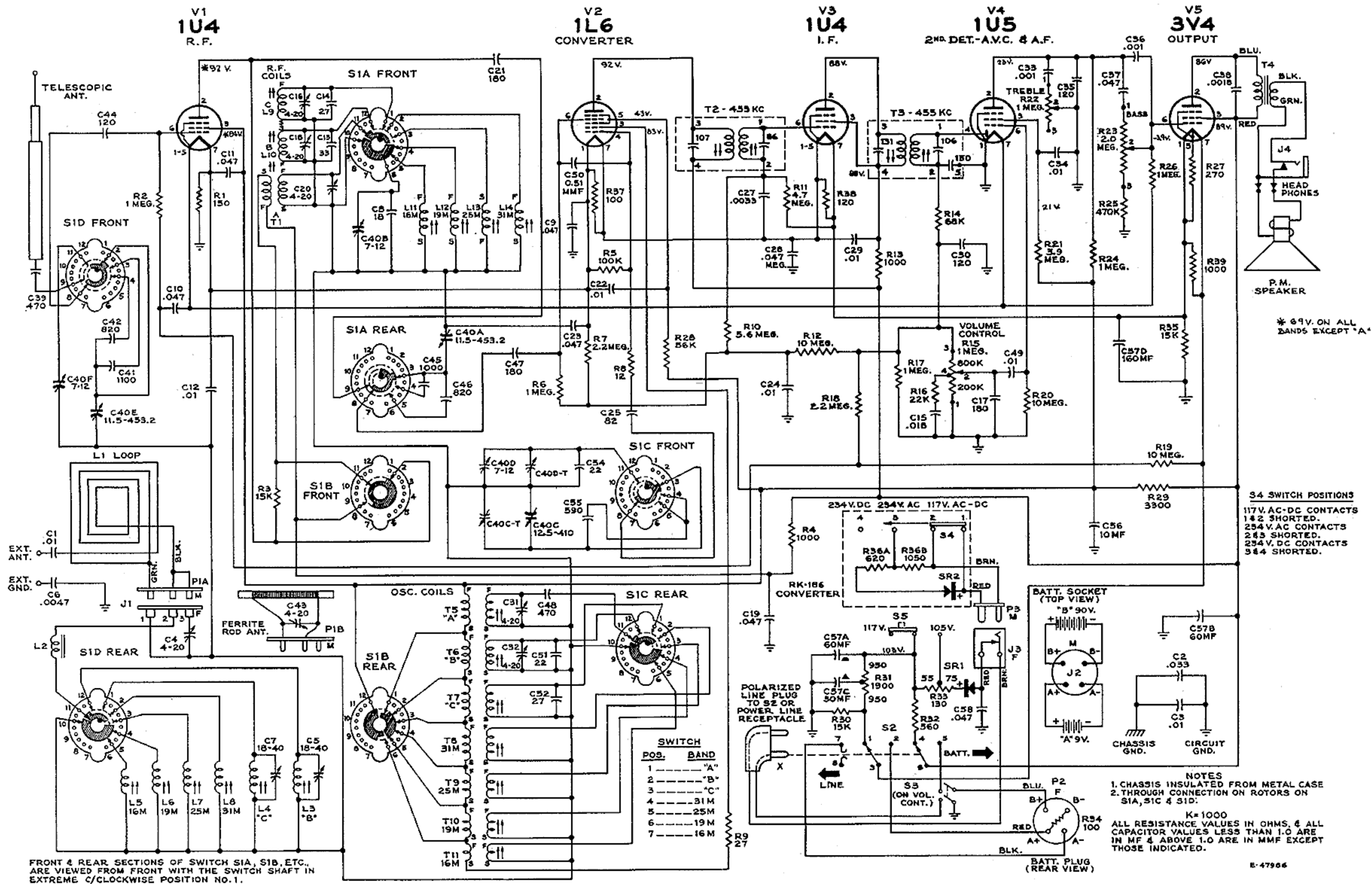
Schematic Diagram—Chassis No. RC-1125
