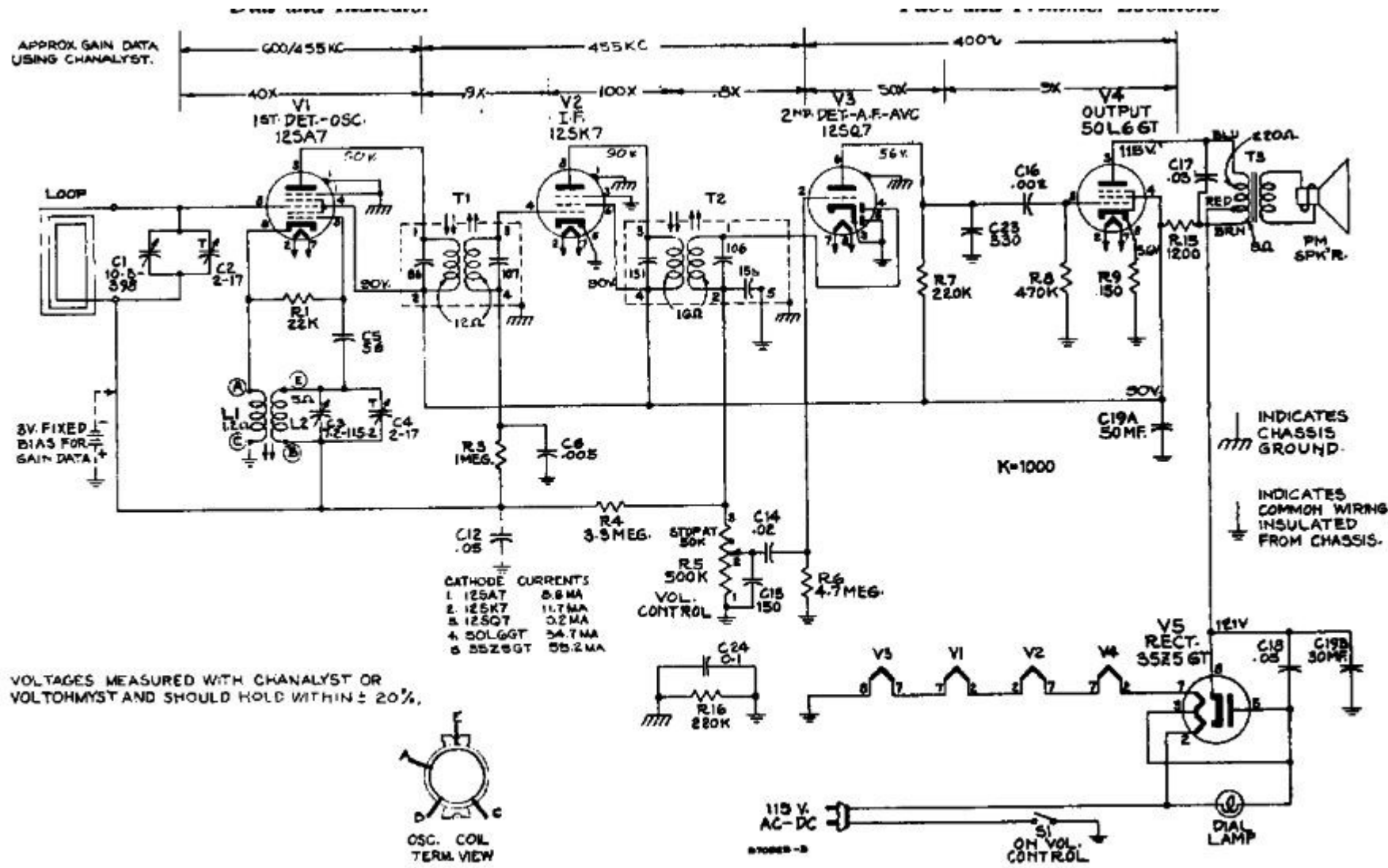
Schematic Circuit Diagram
