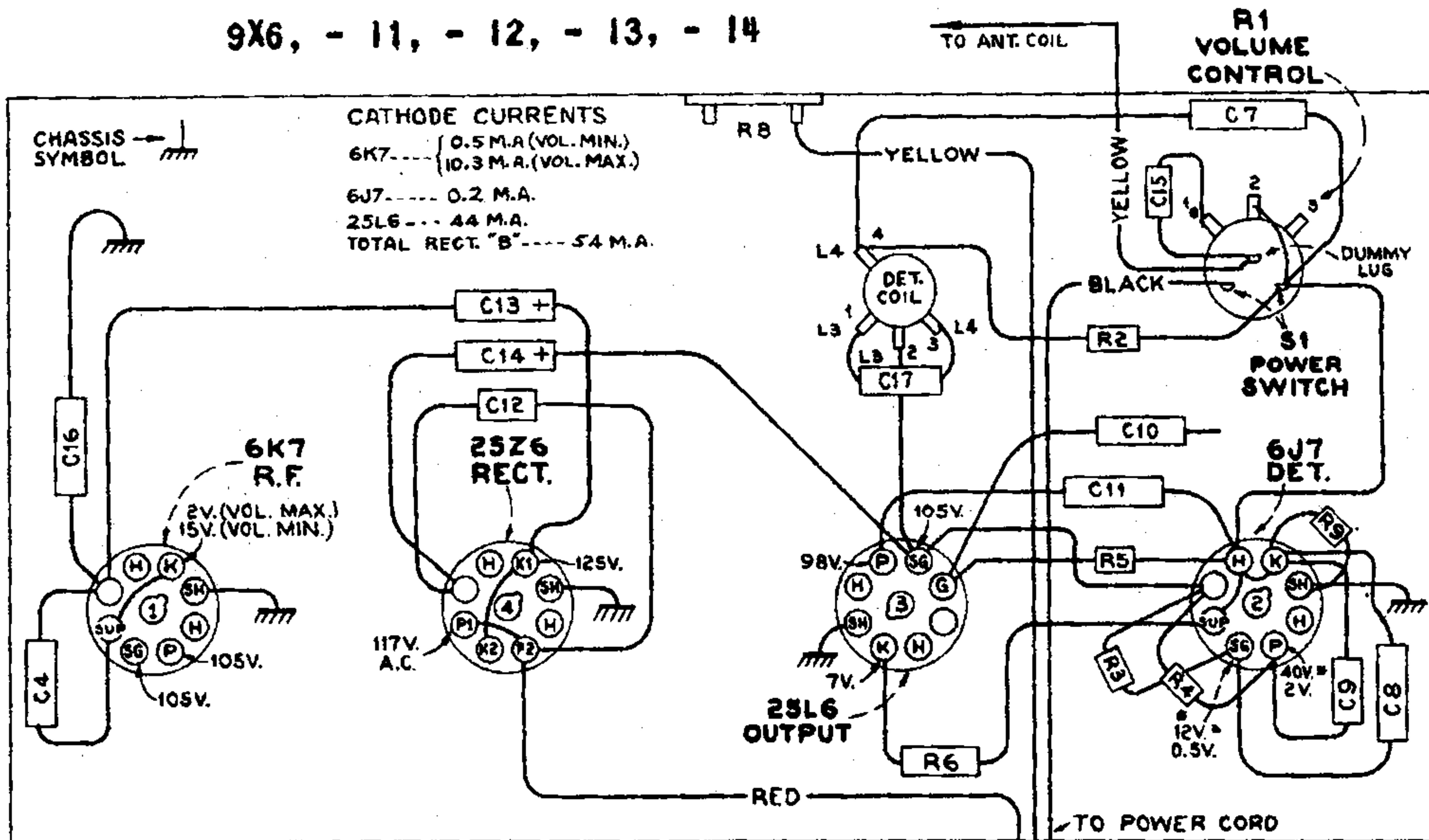
Schematic Circuit Diagram
