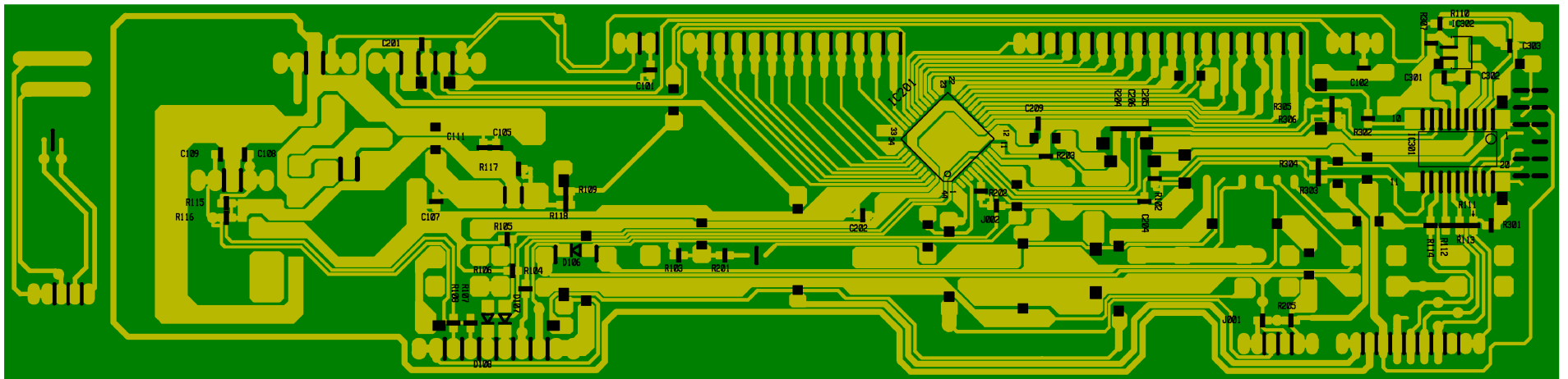
FPA CIRCUIT BOARD (Bottom view)
