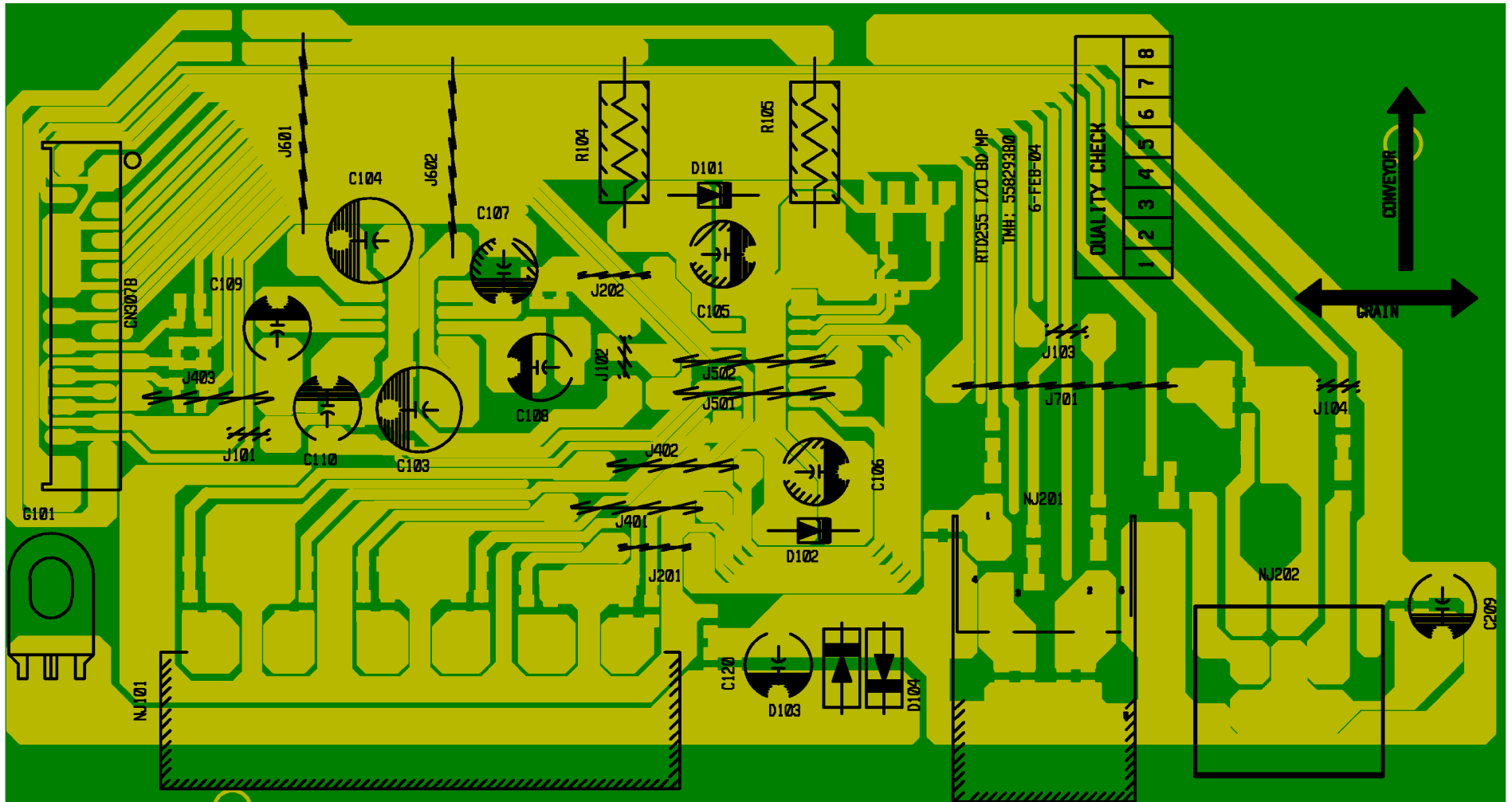
I/O CIRCUIT BOARD (Top view)
