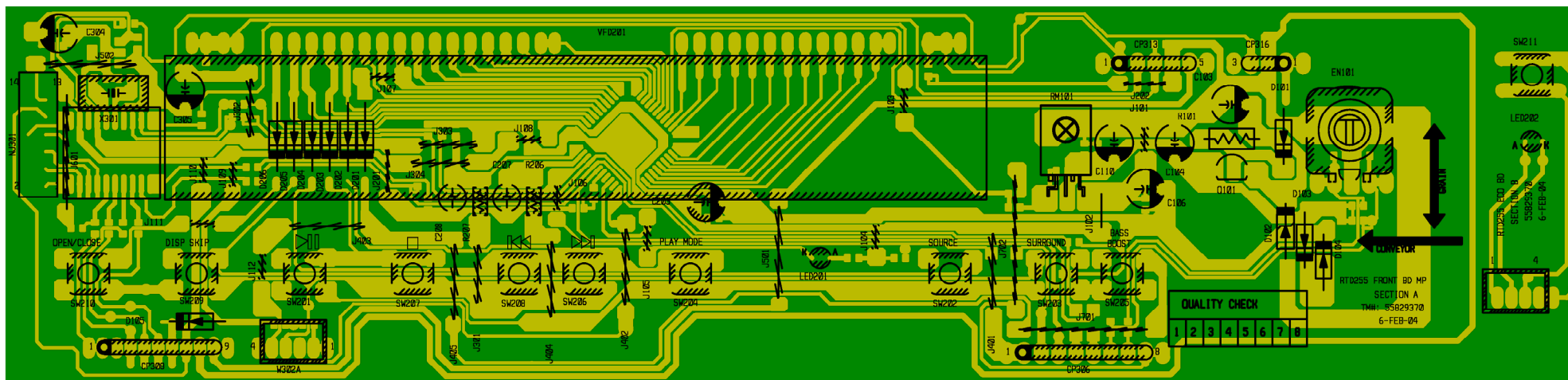
FPA CIRCUIT BOARD (Top view)
