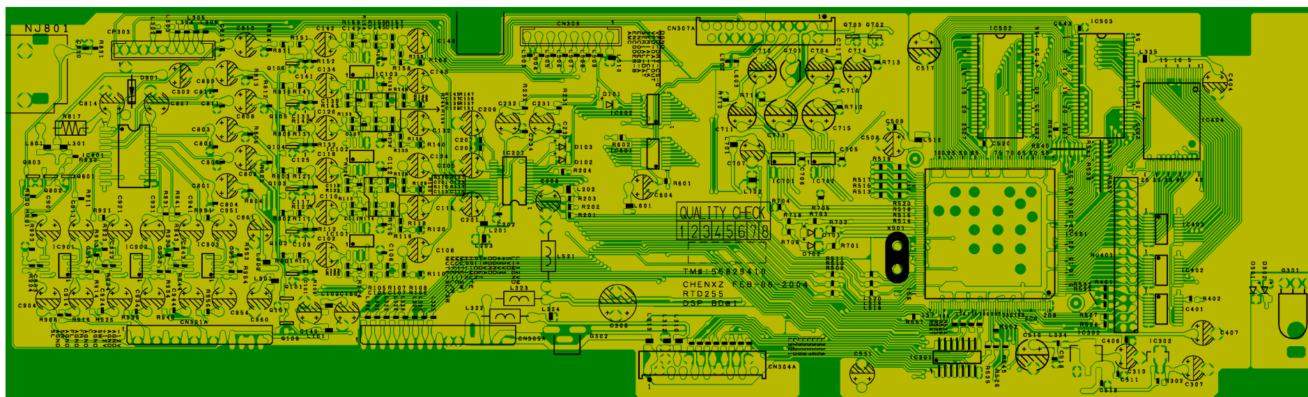
DSP CIRCUIT BOARD (Top view)
