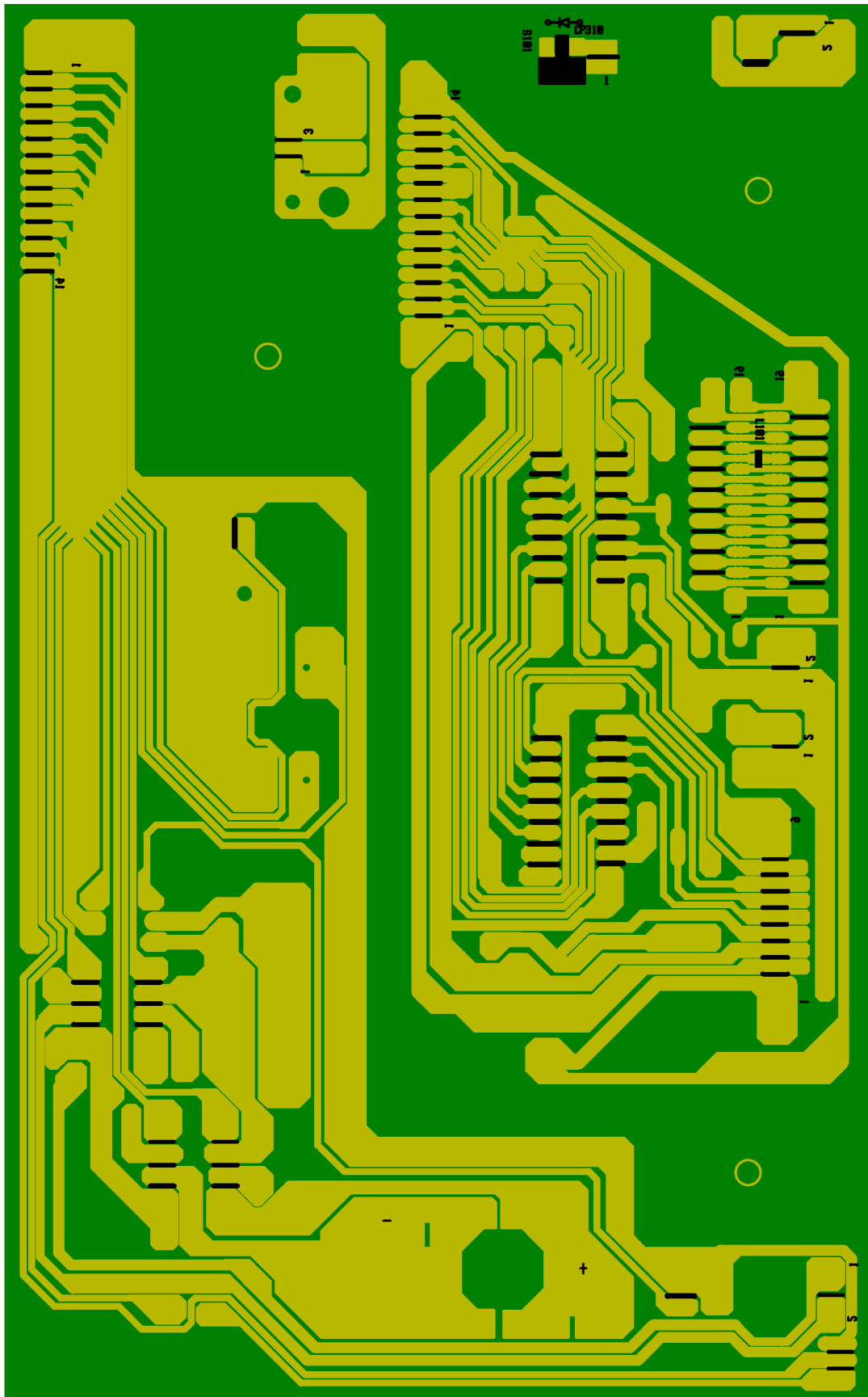
CD DRIVER CIRCUIT BOARDS (Bottom view)
