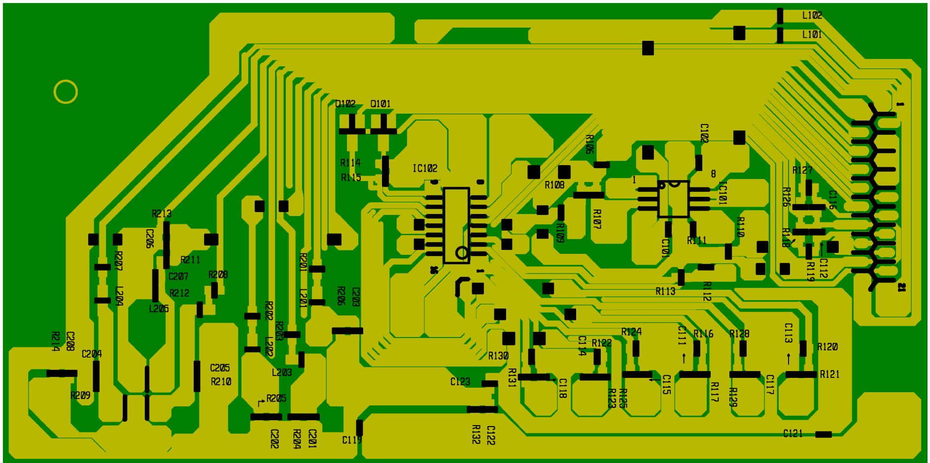
I/O CIRCUIT BOARD (Bottom view)
