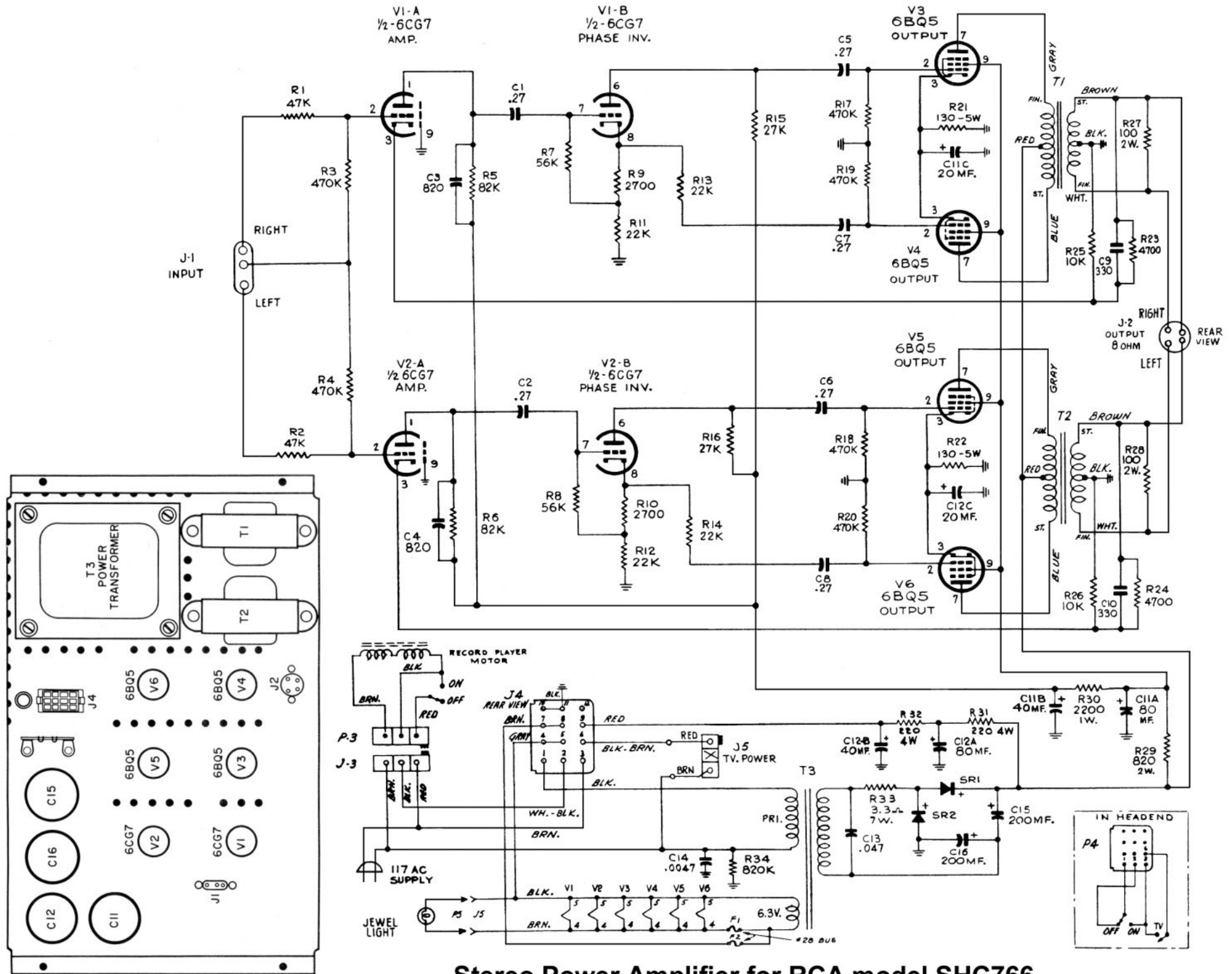
Stereo Power Amplifier for RCA model SHC766
