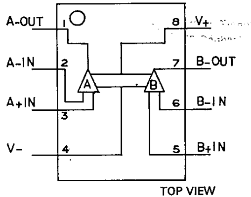
BLOCK DIAGRAM
