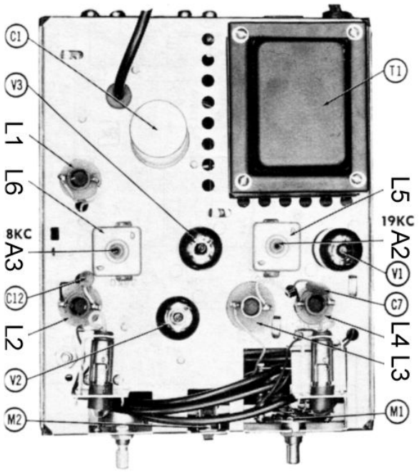
MULTIPLYX ALIGNMENT USING FM STEREO GENERATOR AND AUDIO OSCILLATOR
