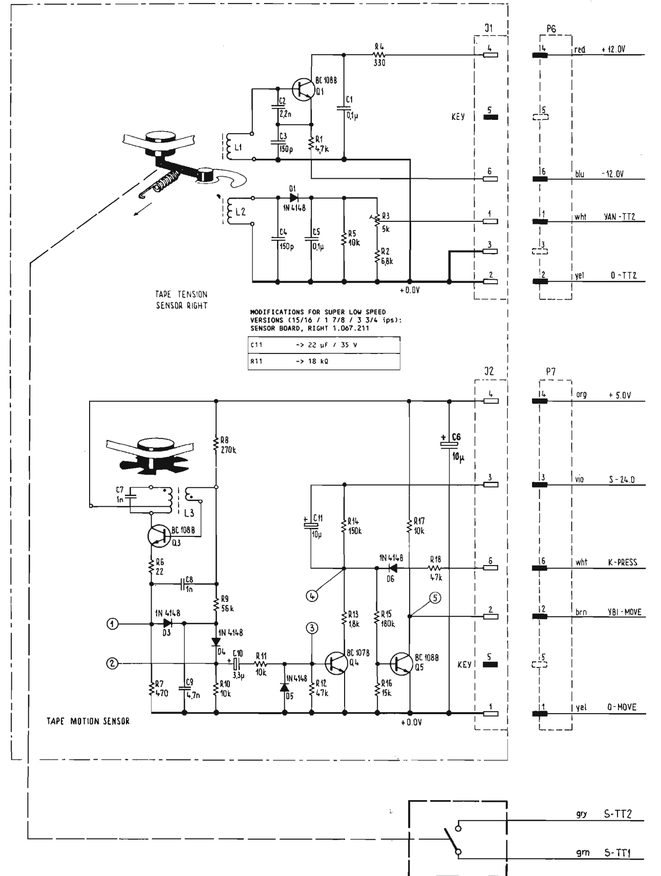
A 7 Sensor board, right Abtasterprint, rechts Circuit analyseur, droit 1.067.210 1.067.211 (SLS)
