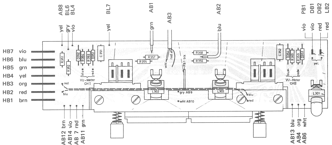
VU-Meter Board 1.077.468
