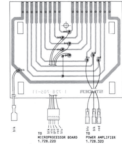
DISTRIBUTOR BOARD SEC. 1.728.705
