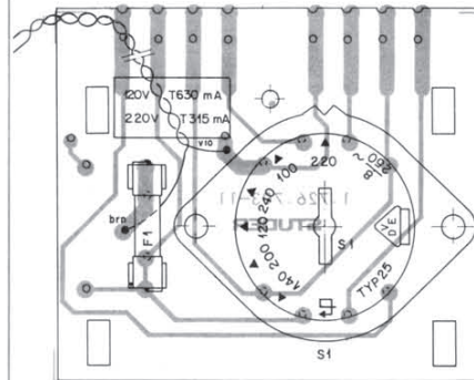
VOLTAGE SELECTOR BOARD 1.728.703
