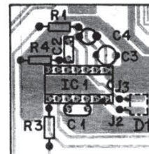
IR SENSOR/RECEIVER
