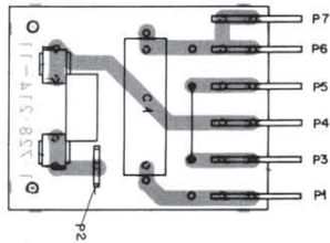
220 V AC POWER SET VERSION: DISTRIBUTOR BOARD 1.728.214
