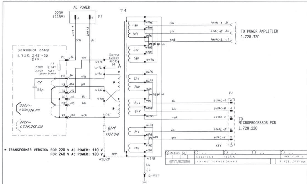
220 V AC POWER SET VERSION: DISTRIBUTOR BOARD 1.728.214
