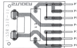
115 V AC POWER SET VERSION: DISTRIBUTOR BOARD 1.728.215
