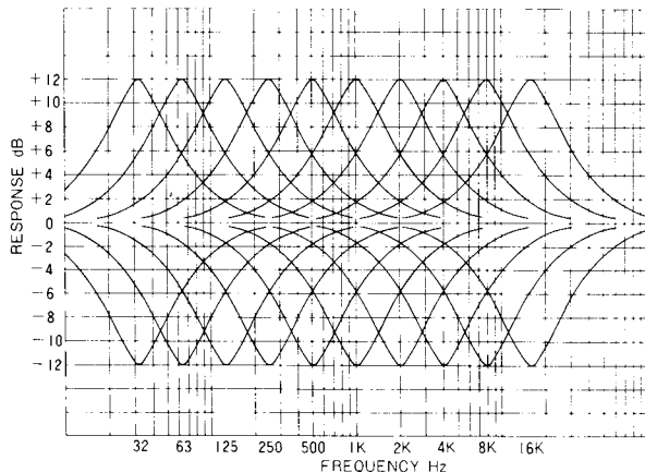
Fig. 1 Frequency Response
