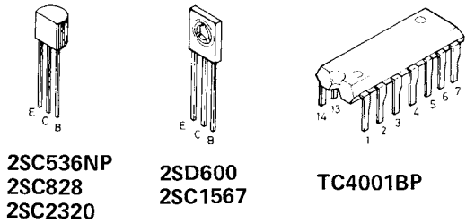
SCHEMATIC DIAGRAM Modle RP-700 1981-03-18 ROTEL
